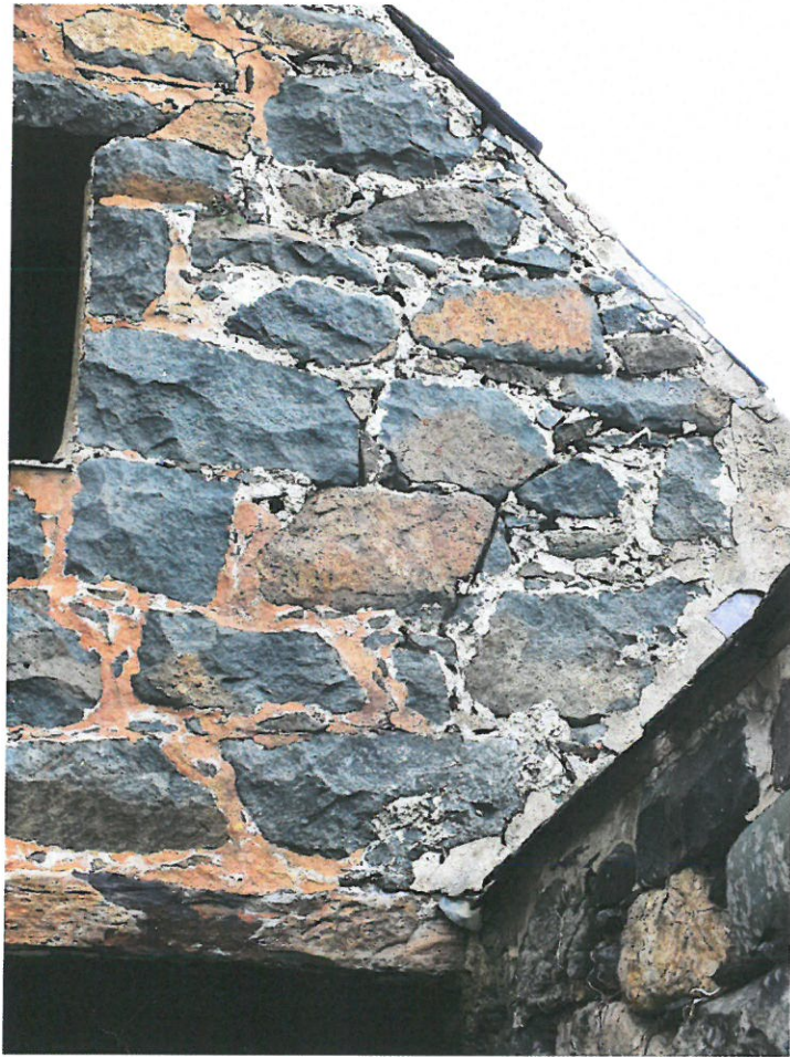
South-West Elevation – Area B – Vertical Cracking
