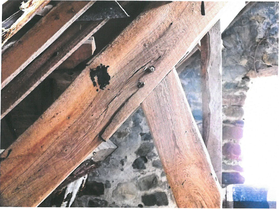
31 Area A – Truss 1
