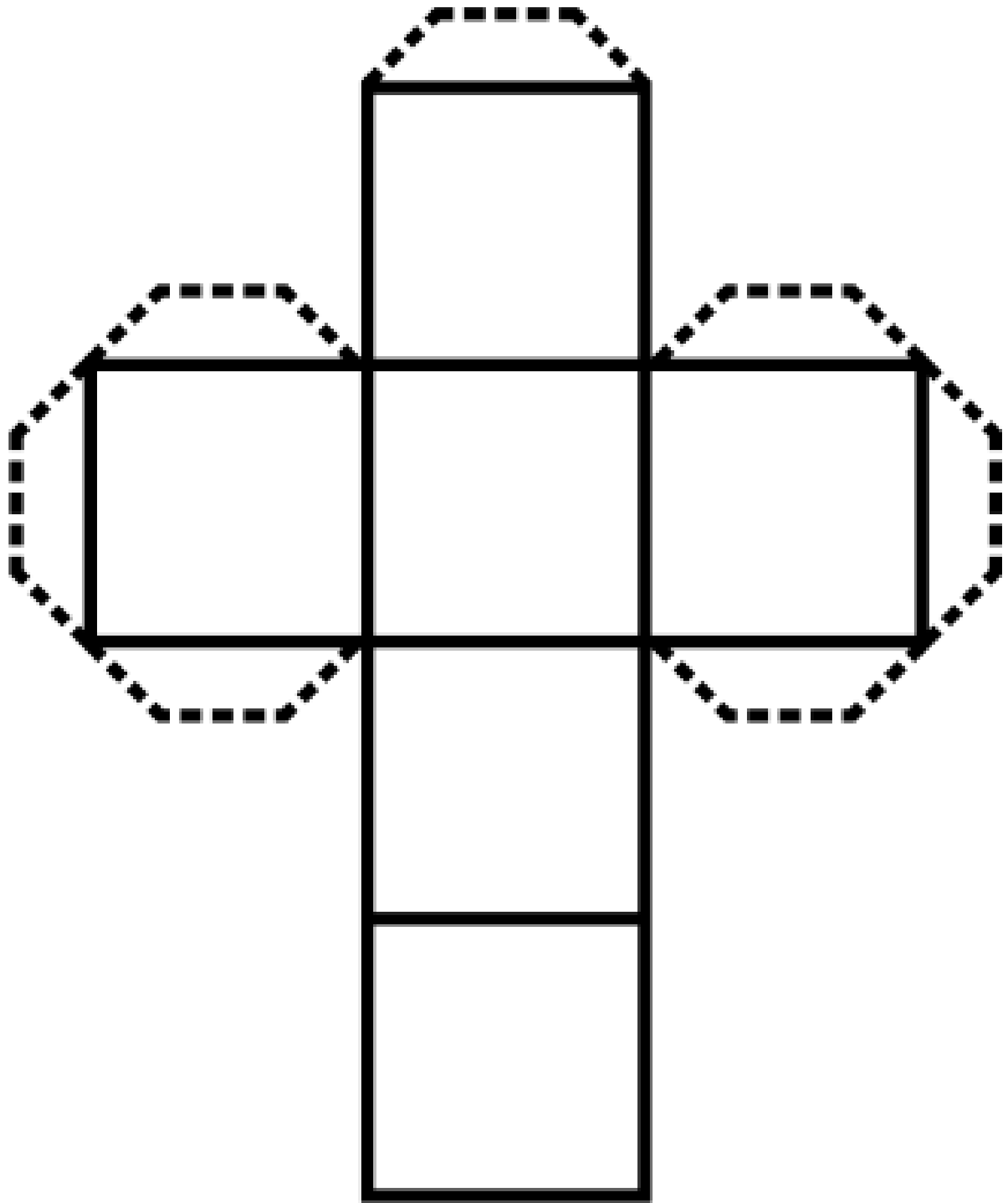
Cube
