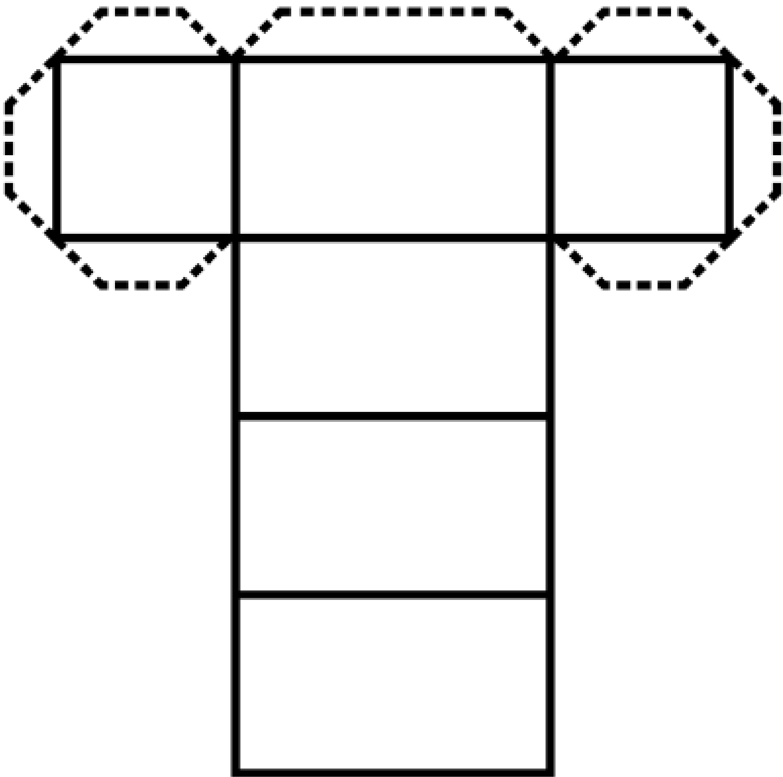
Regtangular Prism
