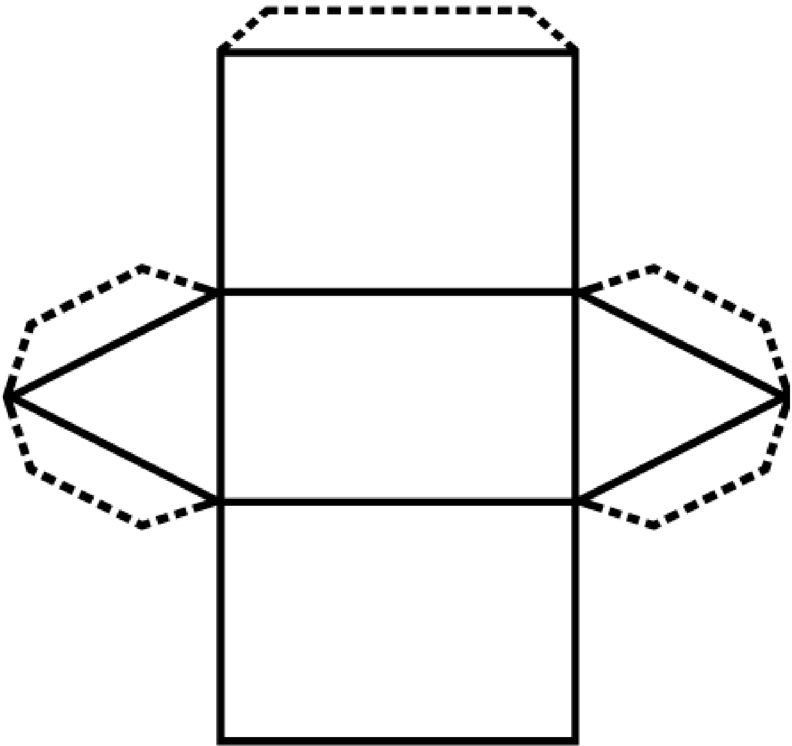
Triangular Prism
