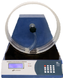
FRIABILITY APPARATUS
