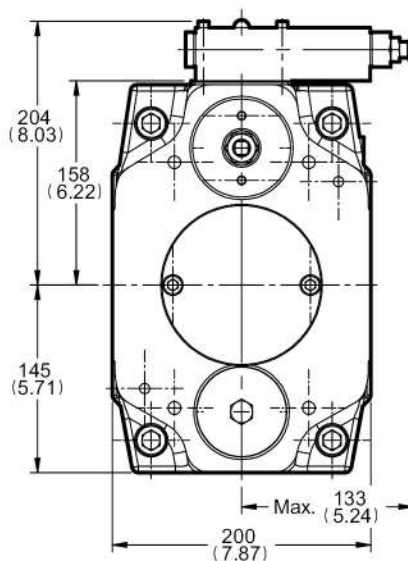
View X
