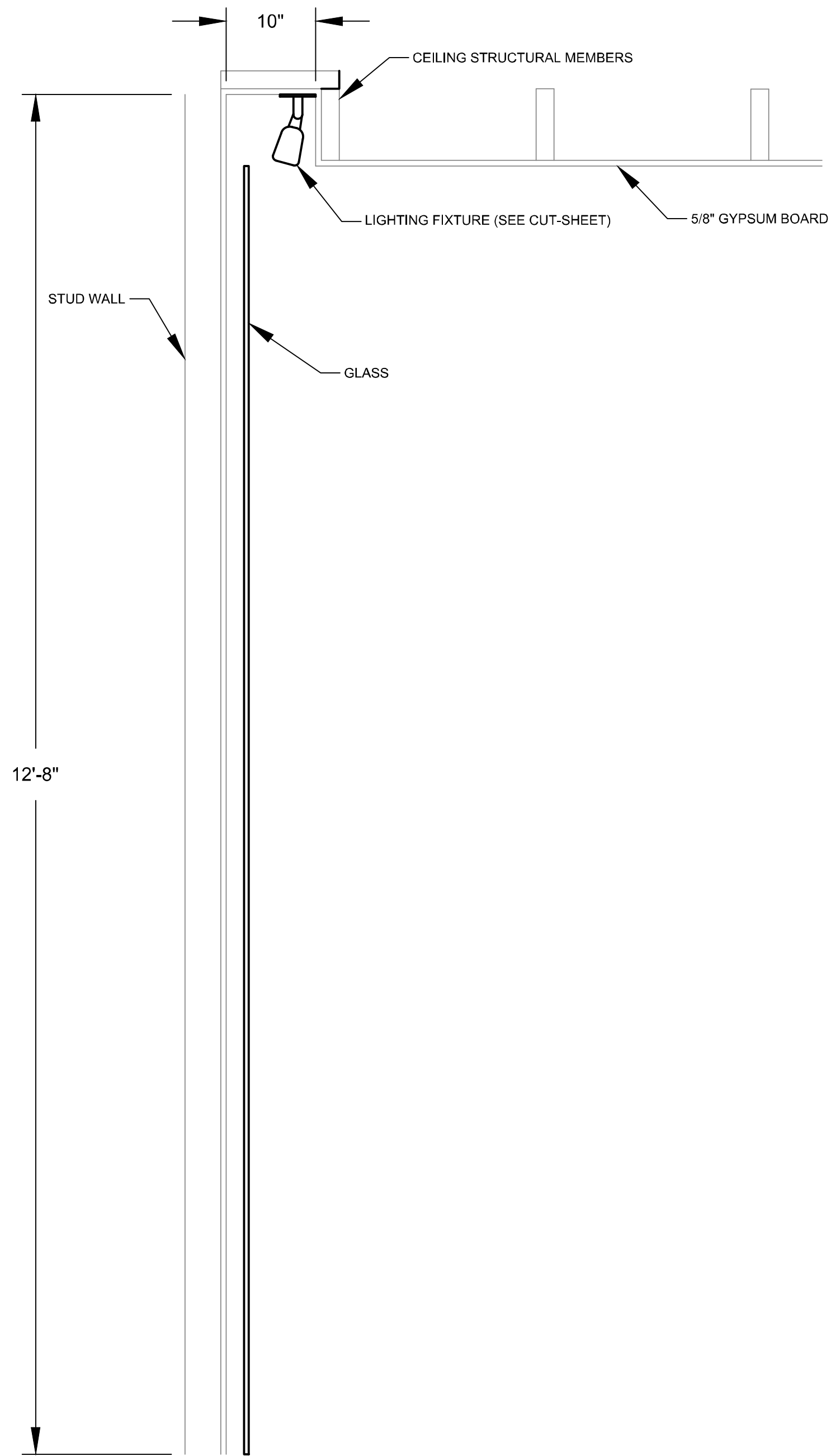
1 HYDREL 4750 - MOUNTING DETAIL 1" = 1'
