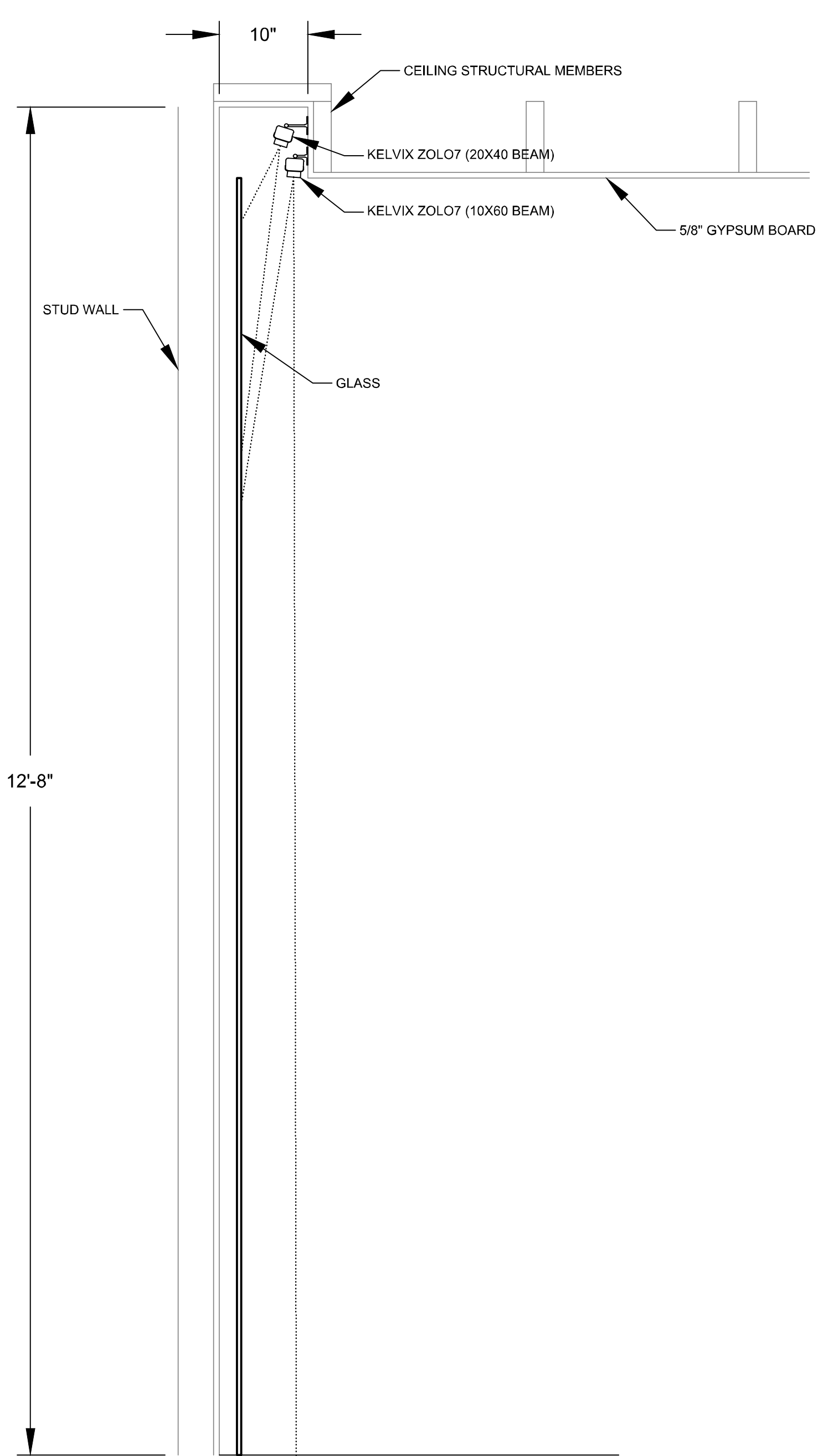
2 KELVIX ZOLO7 - MOUNTING DETAIL 1" = 1'
