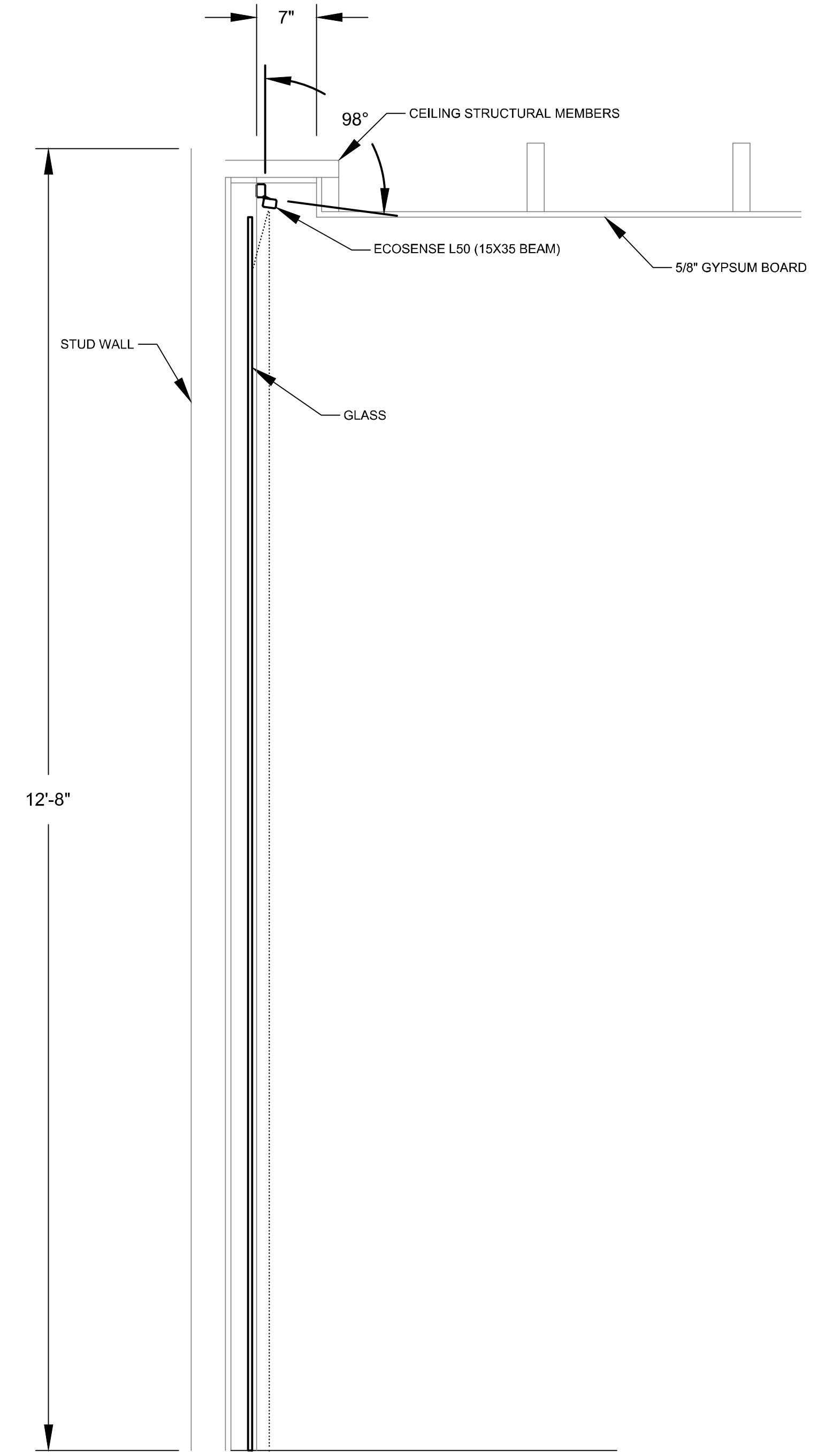
3 ECOSENSE TROV - MOUNTING DETAIL 1" = 1'
