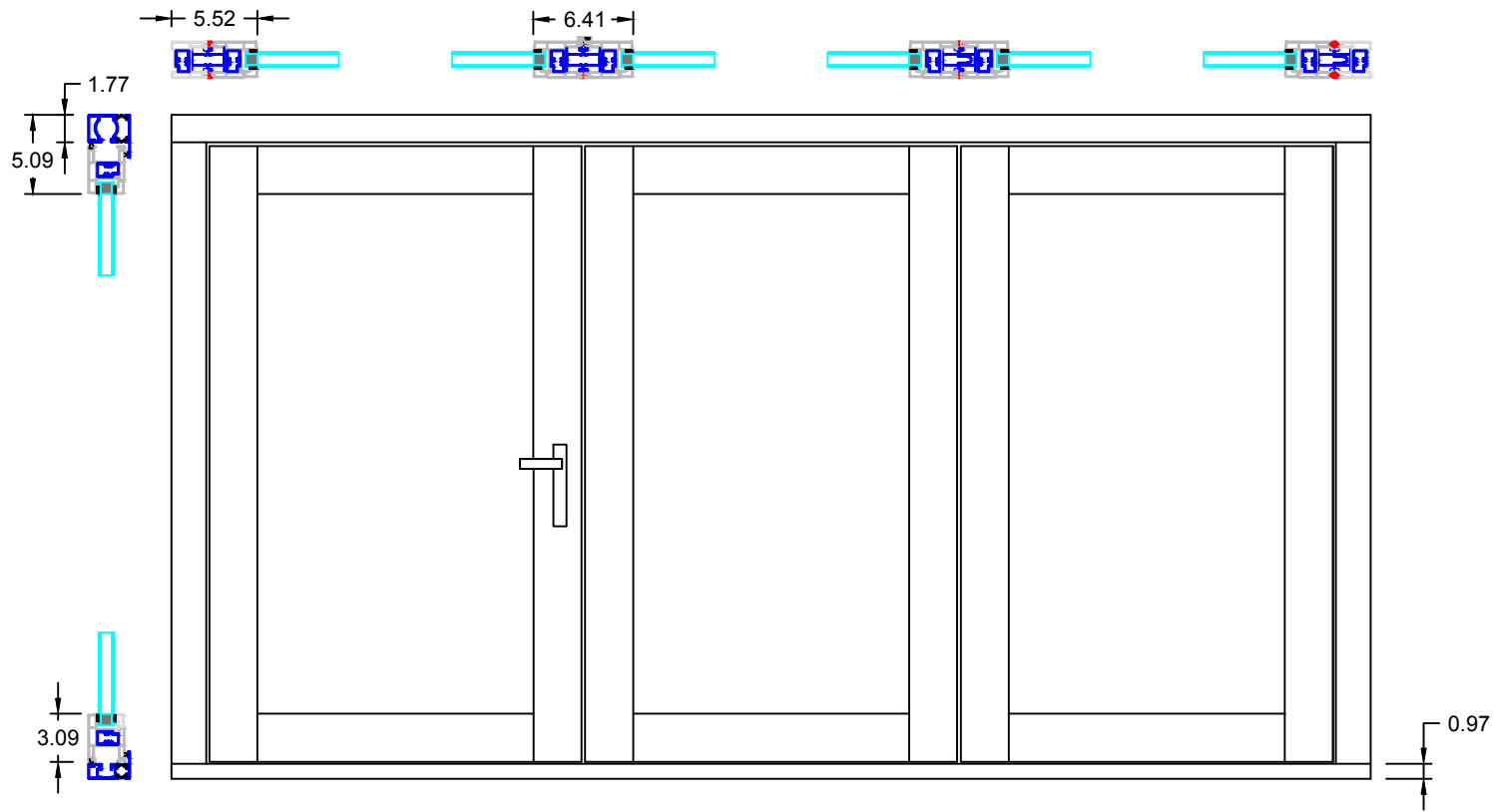
SHOP DRAWINGS ABSOLUTE VINYL SYSTEM ALUMINUM BLOCK FRAME WITH ALUMINUM TRACKS. SIZES ARE IN INCHES.
