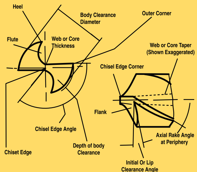
NOMENCLATURE OF TAPER SHANK DRILL
