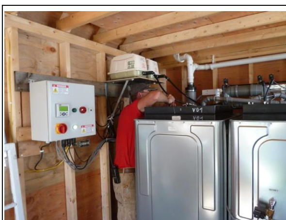
Installation of the BUSSE-MF in the shed
