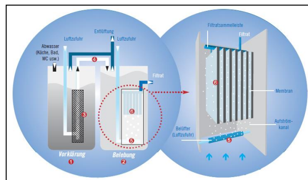
Process design of the BUSSE-MF technology
