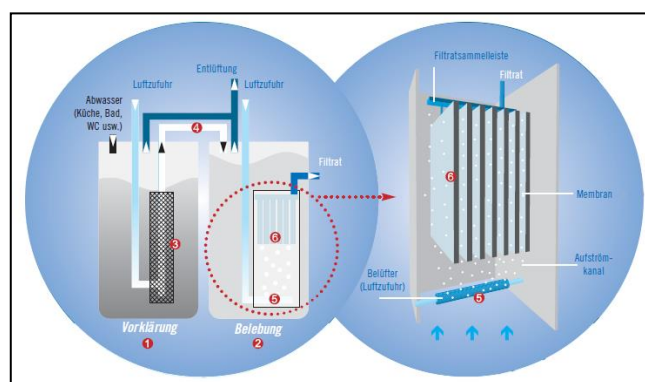
Process design of the BUSSE-MF technology
