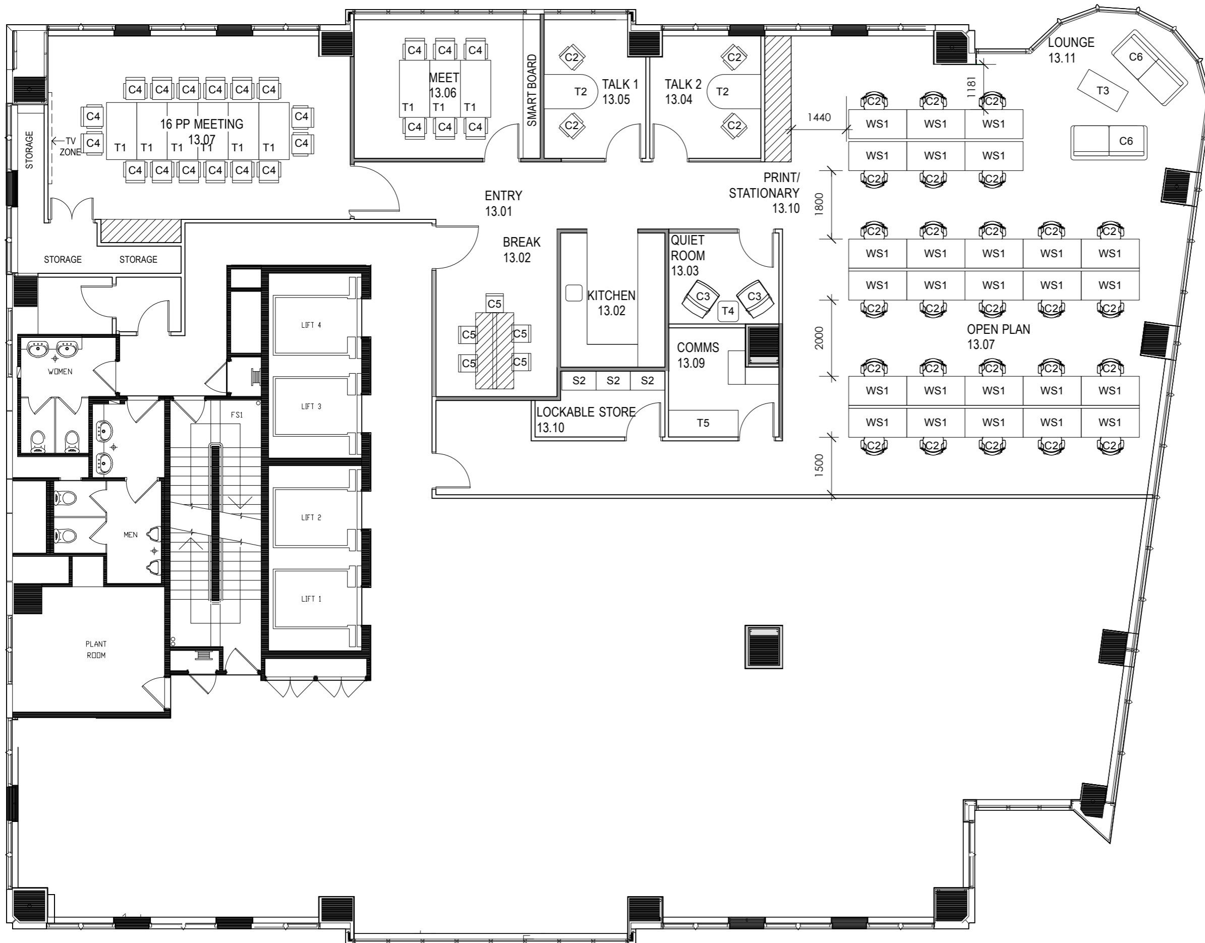
1 FURNITURE PLAN 1:100 @ A3
