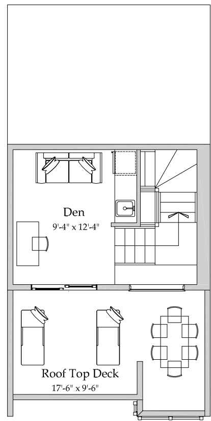
LOFT LEVEL
