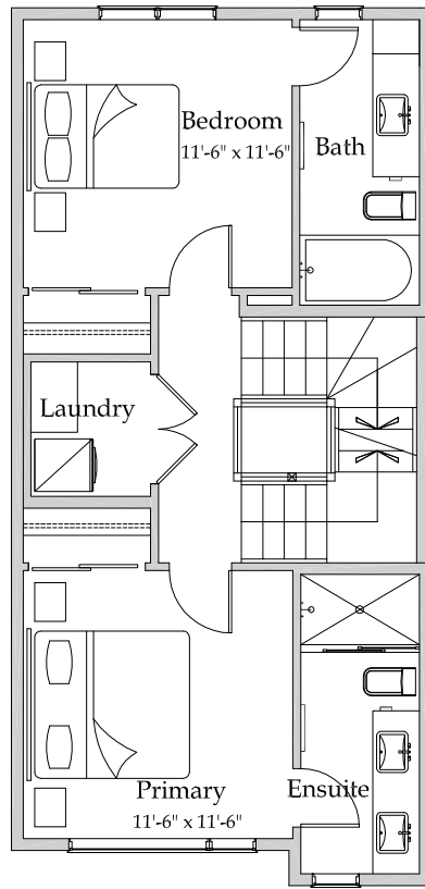
UPPER LEVEL
