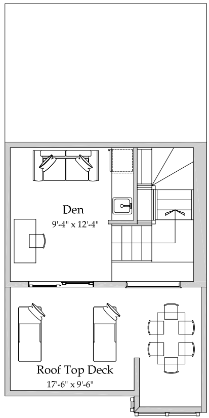
LOFT LEVEL
