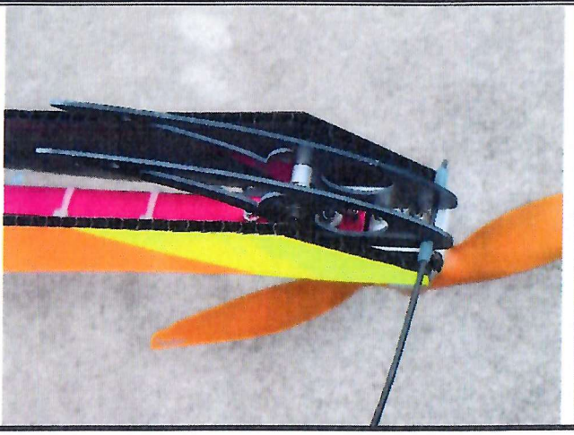
$75 Stunt Quad, Spring loaded Landing Gear, KK controller. Capable of flips, rolls and tumbles. Color scheme for orientation.
