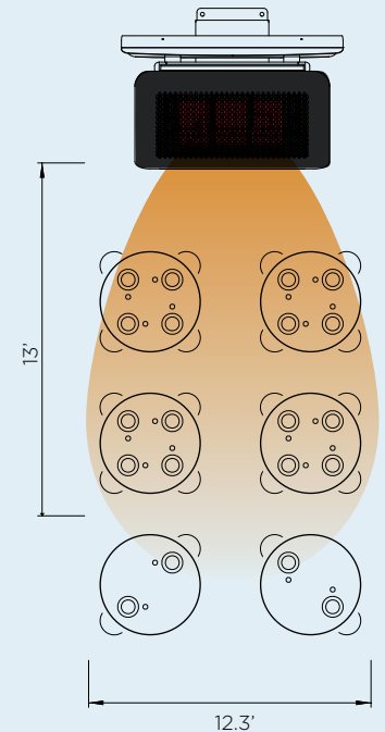
HEATING APPROXIMATELY 160FT 26,000 BTU HEATING POWER
