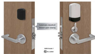
e-CRONUS 1A Automatic Deadbolt
