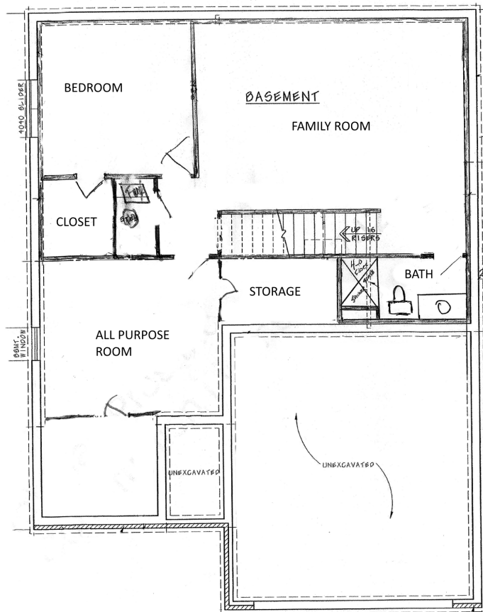
FOUNDATION PLAN
