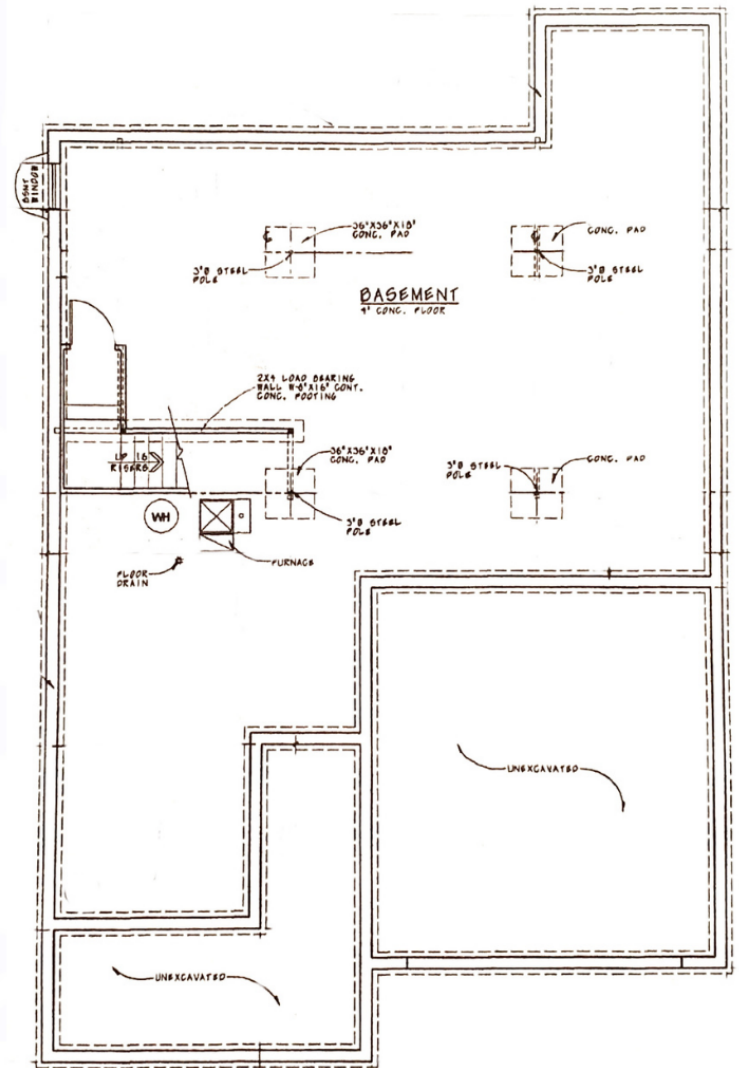
BASEMENT LEVEL
