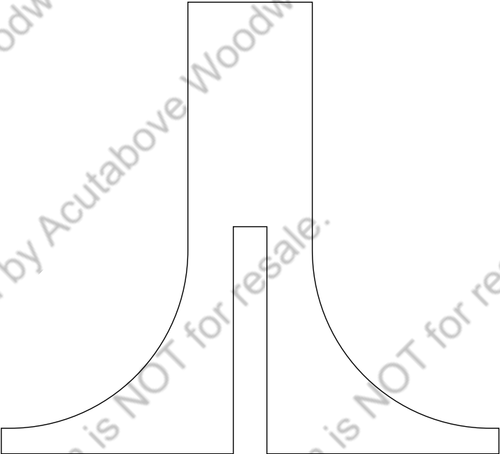
Leg Pedestal. Make 1 from 1/4" thick stock
