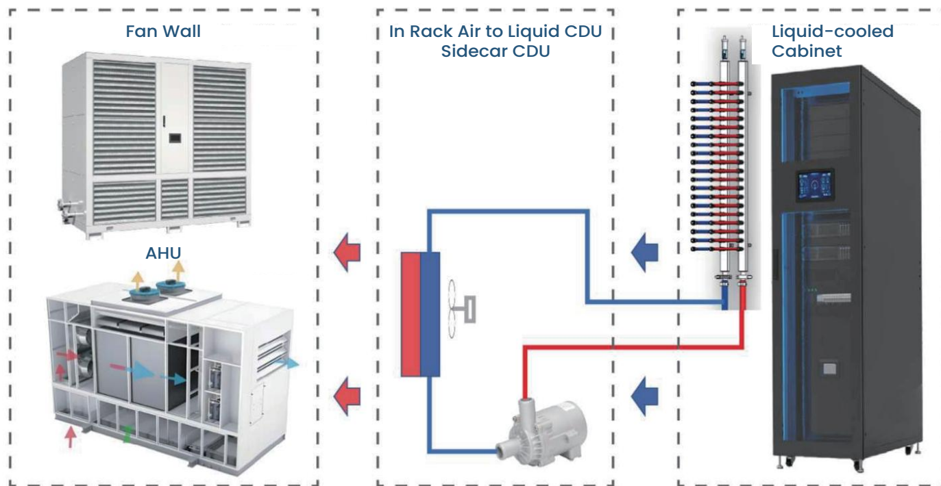
* A2L Retrofit System Schematic
