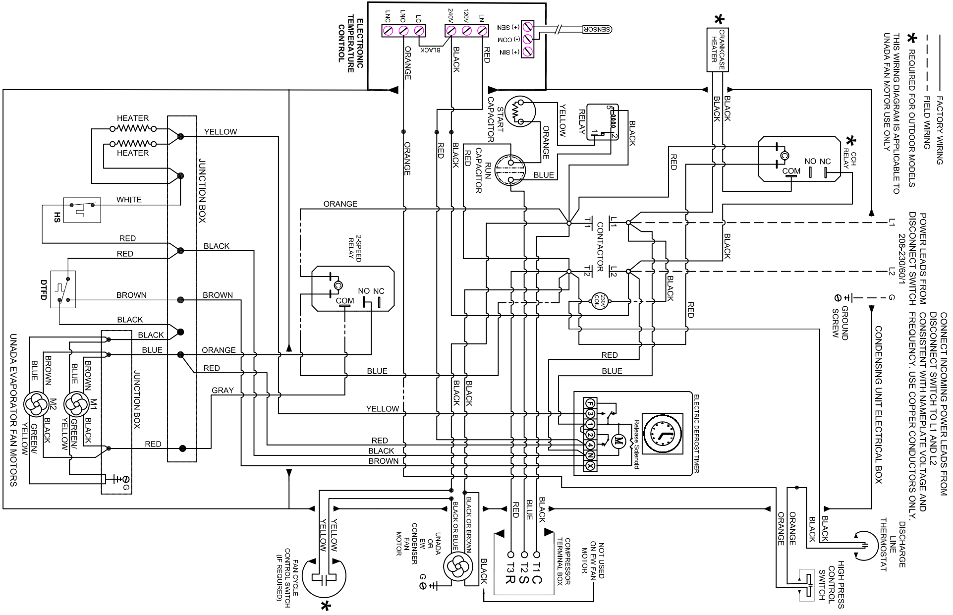
R448A POLAR PAK FREEZER WIRING DIAGRAM 208-230/1/60
