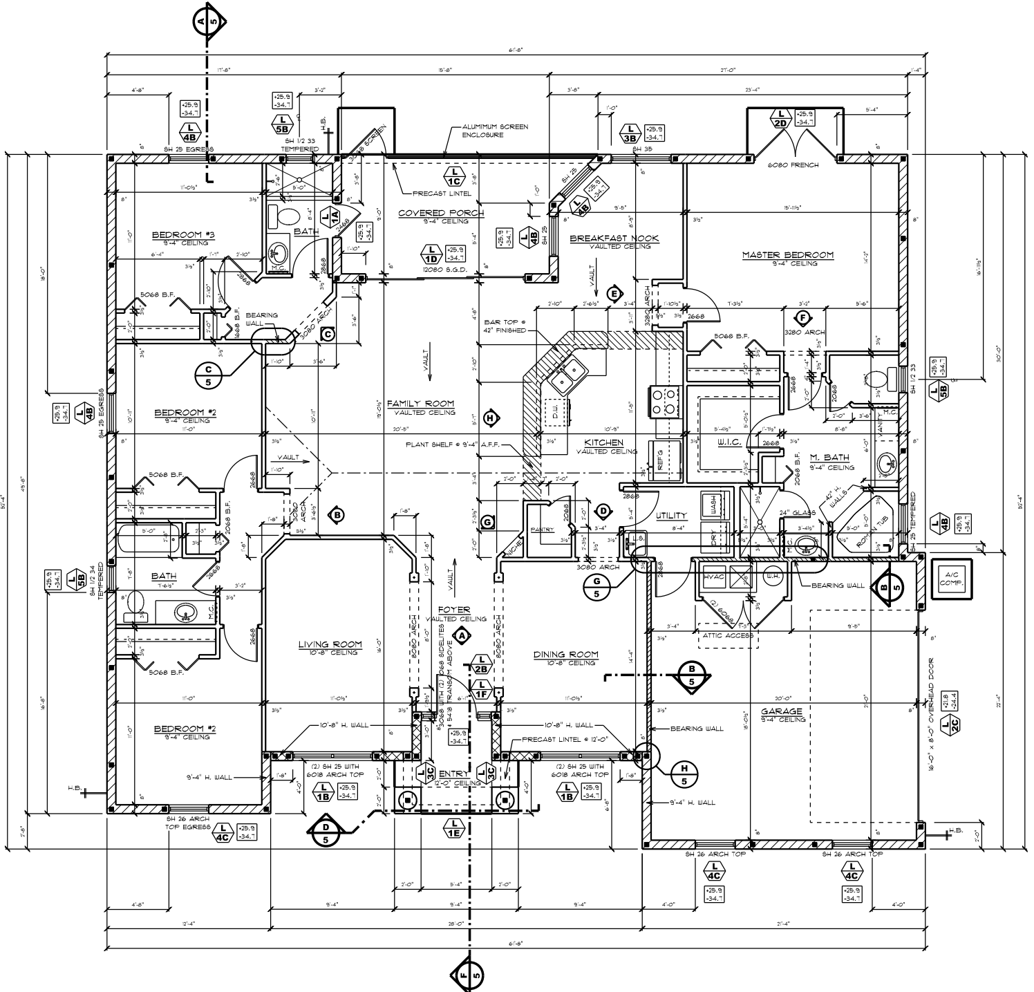
FLOOR PLAN
