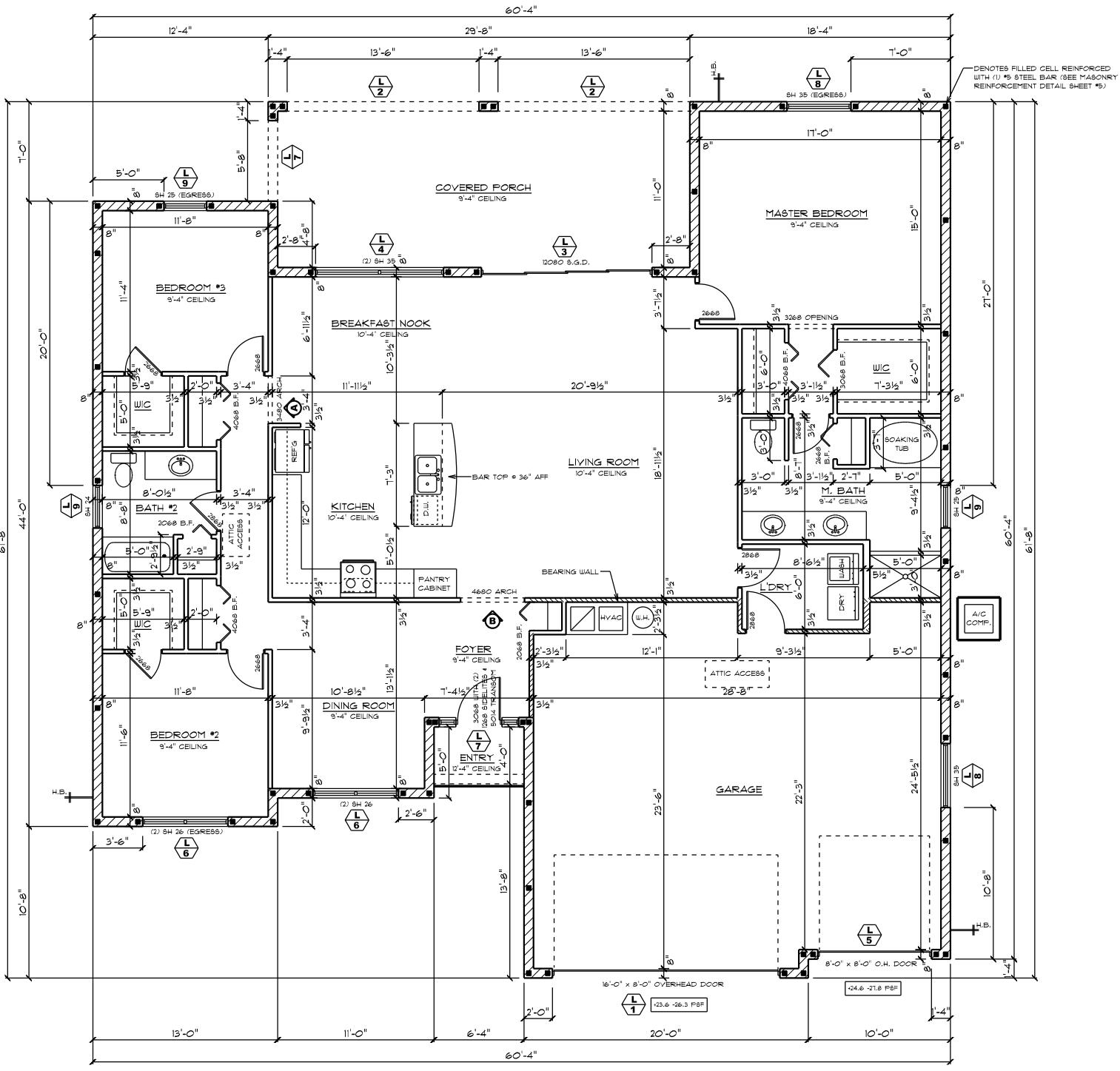
FLOOR PLAN
