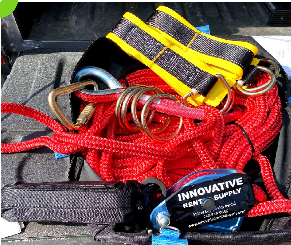
Horizontal and Vertical Lifelines Improve Efficiency By Extending Your Access
