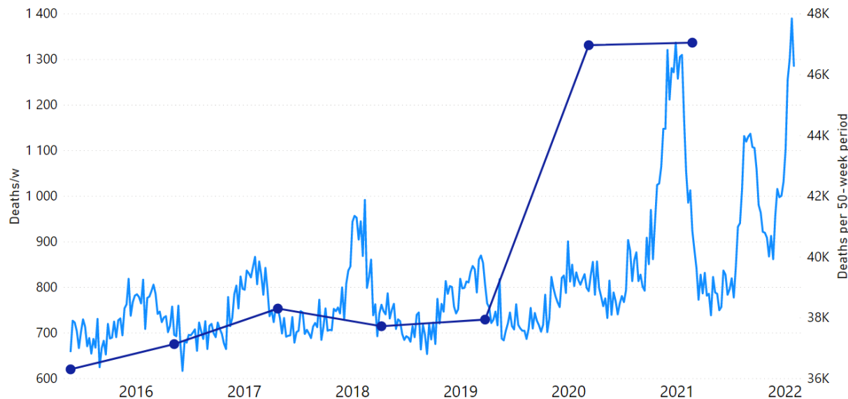
ACM/w, Oklahoma, 2015-2022
