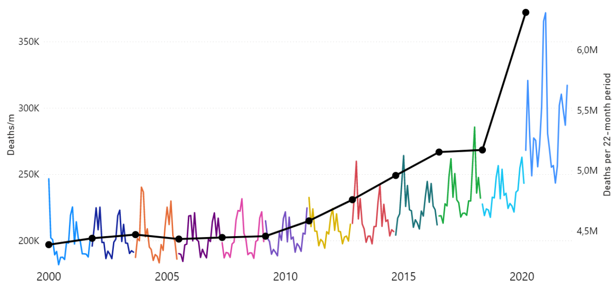
ACM/m, USA, 2000-2021
