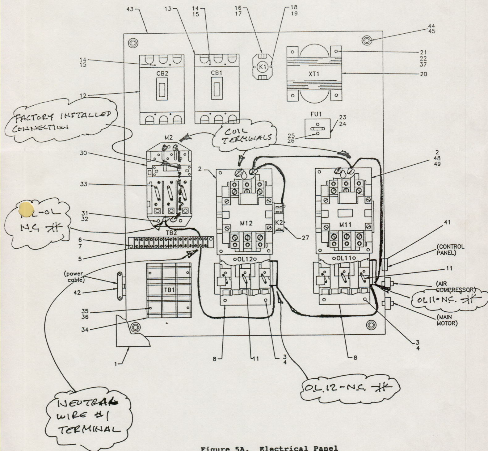
Figure 5A. Electrical Panel
