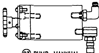
③ PUMP, MANNUAL SCREW ASSY (1) P2C02B001A
