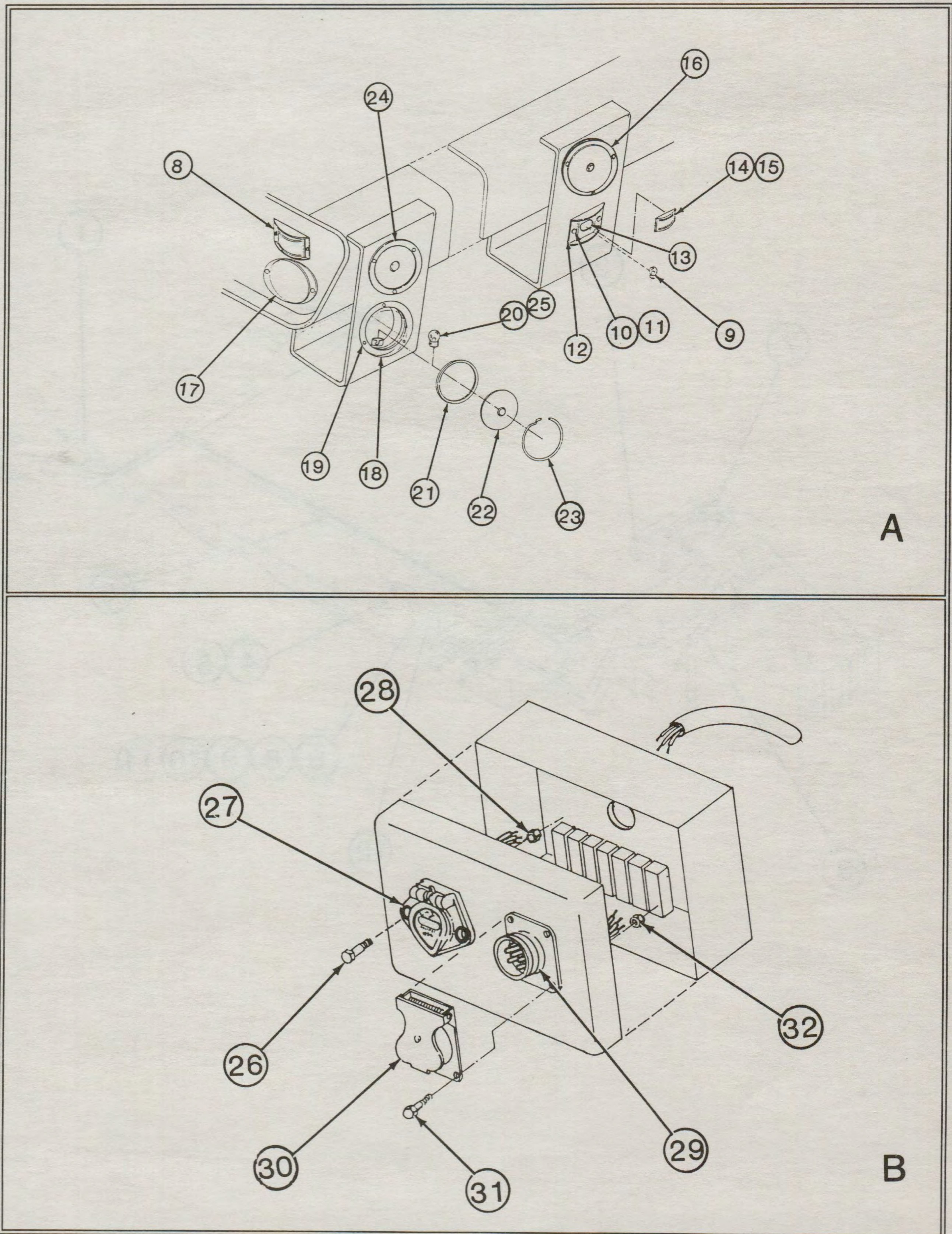
4-10.1 LIGHTS, REFLECTORS, AND RECEPTACLE ASSEMBLY
