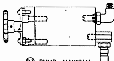
③ PUMP, MANUAL SCREW ASSY
