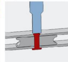
Radial point riveting
