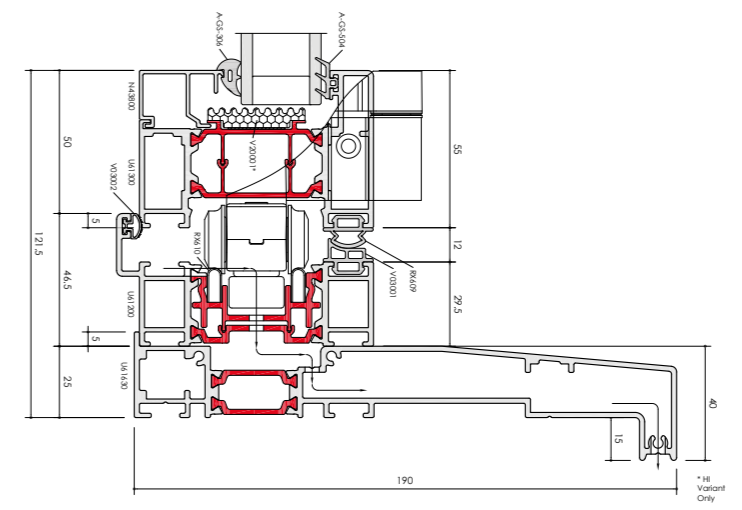
F82 CILL AND SUBCILL / D
