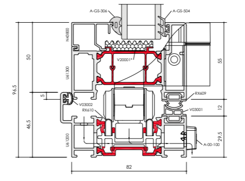
F82 WITH FACE DRAINAGE / D1
