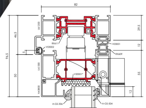
F82 HEAD / A
