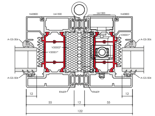
F82 MEETING STYLE / B
