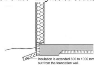
Slab On Grade - Engineered Structural Slab
