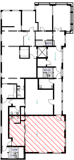
SECOND FLOOR KEY PLAN
