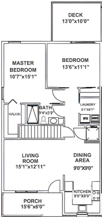
HIGHLAND II MAIN FLOOR
