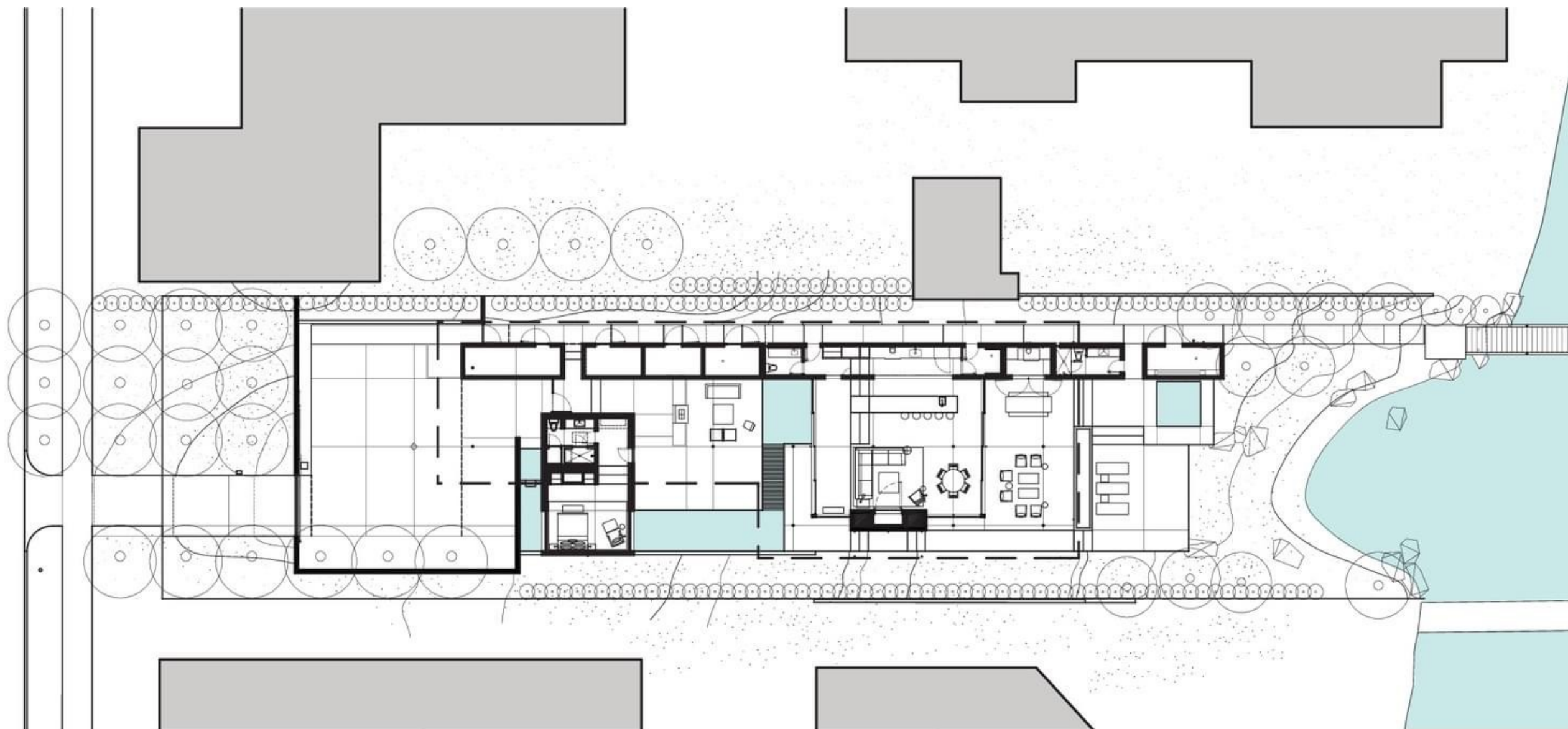
SITE CONTEXT AND FLOOR PLAN
