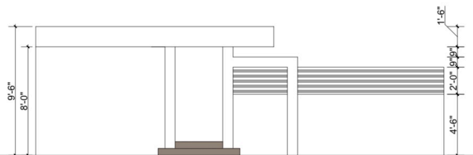
BOUNDARY WALL ELEVATION
