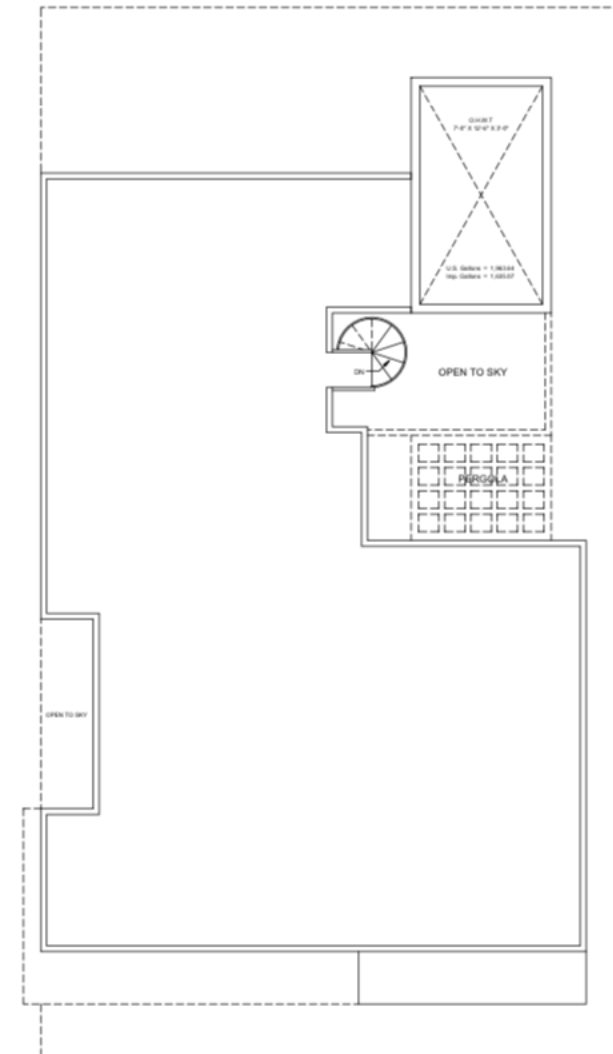
ROOF PLAN
