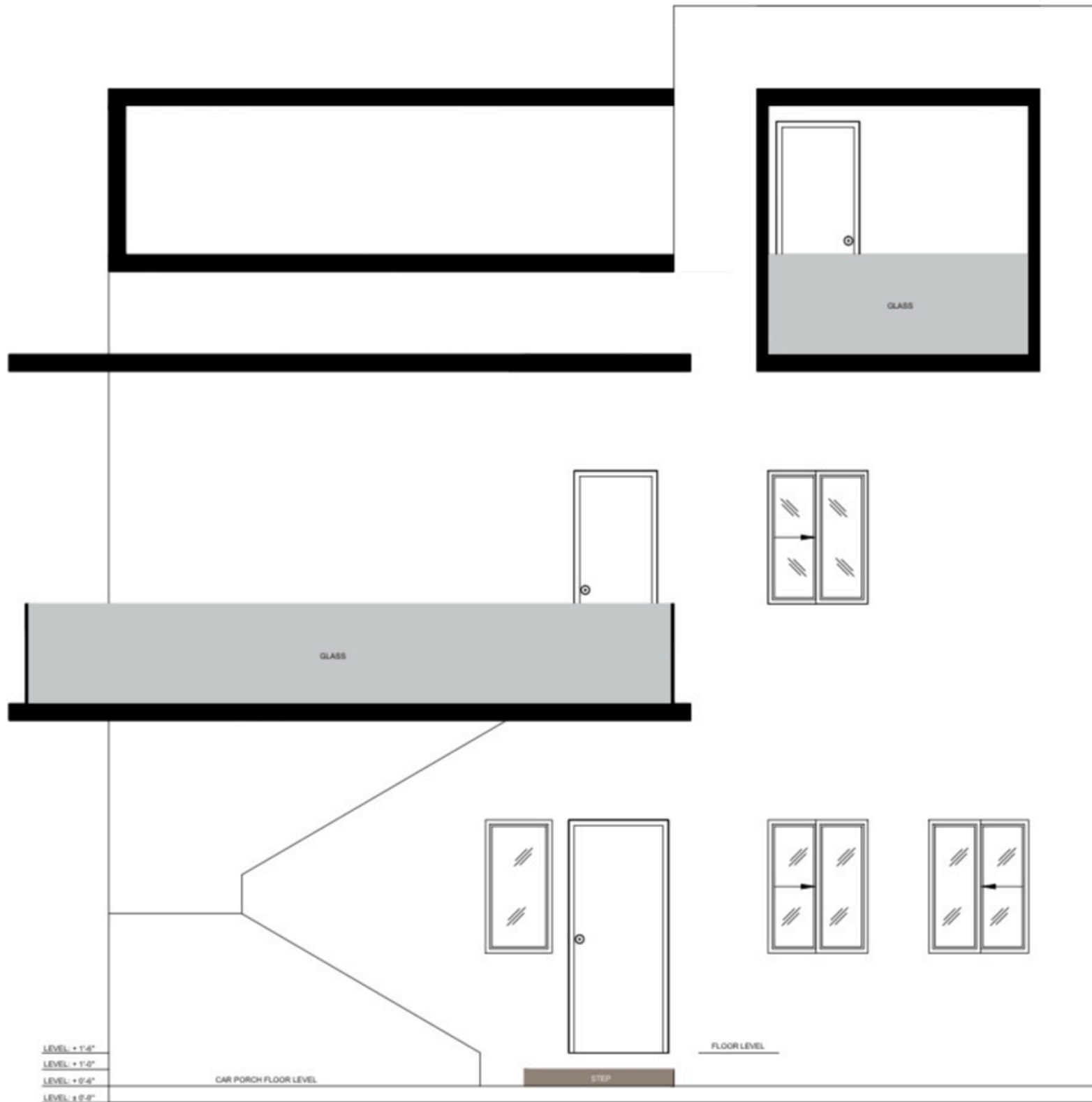
FRONT ELEVATION (ONE UNIT)
