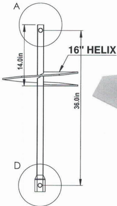
1 1.5" RCS EXTENSION 1" = 1' 0"
