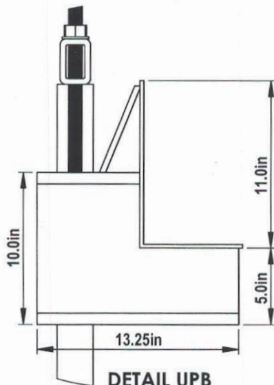
DETAIL UPB SCALE 1 : 8
