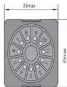
Outside dimensions drawing (NJDC-12/3Z)
