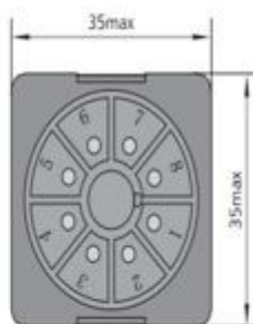
Outside dimensions drawing (NJDC-12/2Z)
