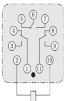
Bottom wiring diagram (NJDC-12/3Z)
