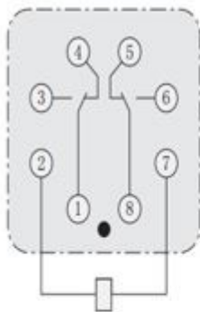
Bottom wiring diagram (NJDC-12/2Z)
