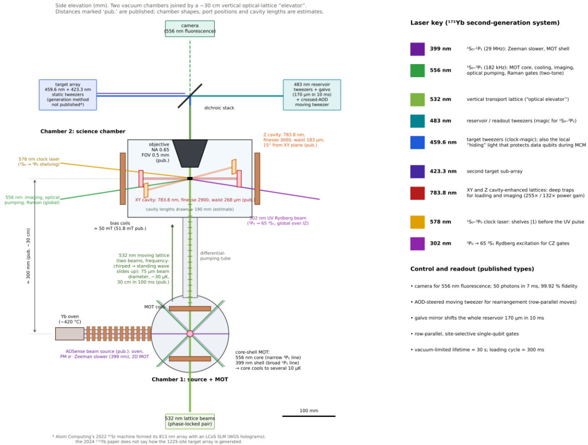
Figure 1. Side elevation of the second-generation ^{171}\text{Yb} system with laser key. The atom source is a commercial AOSense unit, drawn here as its internal oven and slower. The ~30 cm elevator, the cavity finesse, waists and tilt, the NA, the field of view and the bias field are published; chamber shapes, port positions and the drawn cavity length (~190 mm) are estimates.
