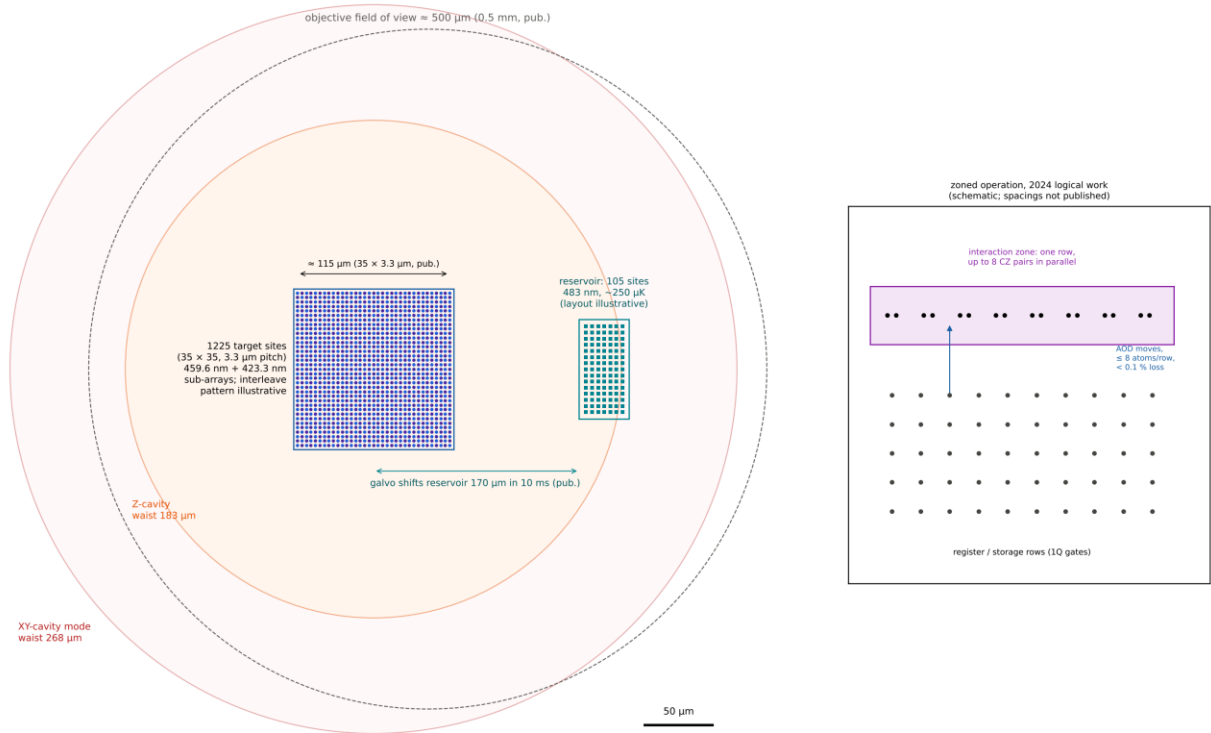
Figure 2. Atom plane in micrometers. The 35 \times 35 target array at 3.3 \mu\text{m} pitch, the 105-site reservoir and its 170 \mu\text{m} galvo shift, the cavity waists and the field of view are published. The interleave pattern of the two target sub-arrays and the reservoir arrangement are illustrative. Right: zoned operation in the 2024 logical work (schematic).
