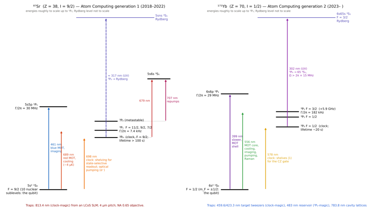
Figure 3. Level diagrams for ^{87}\text{Sr} (Atom Computing generation 1) and ^{171}\text{Yb} (generation 2), with the wavelengths each machine uses. Energies are roughly to scale up to ^1P_1 ; the Rydberg levels are not.
