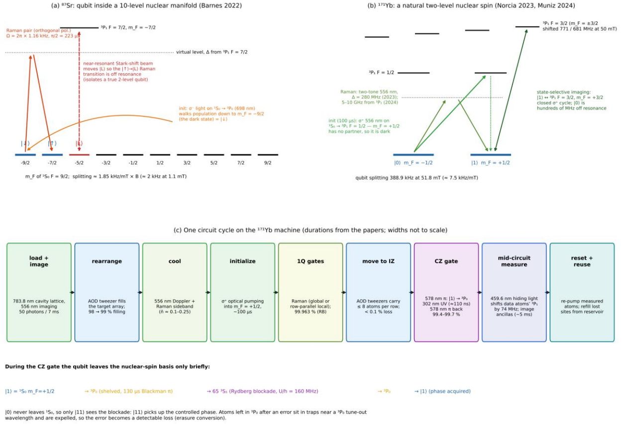
Figure 4. (a) ^{87}\text{Sr} qubit inside its ten-level ground manifold. (b) ^{171}\text{Yb} qubit with the transitions used for pumping, Raman gates and state-selective imaging. (c) One circuit cycle on the ^{171}\text{Yb} machine.
