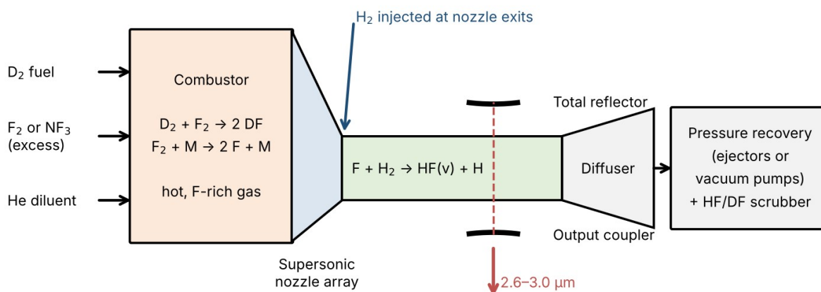
Figure 5. Layout of a continuous-wave supersonic-mixing HF chemical laser. The optical axis runs across the flow; the D_2 combustor supplies hot F atoms, H_2 is injected at the nozzle exits, and HF(v) is formed and lases in the mixing zone before the gas is slowed in the diffuser and pumped away.
