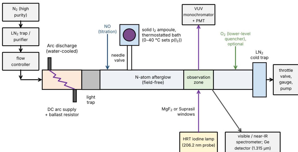
Figure 10. Proposed nitrogen-afterglow apparatus for studying the \text{N} + \text{NI} reaction. N atoms made in a water-cooled DC arc pass through a light trap into a field-free, \text{H}_3\text{PO}_4 -coated flow tube. Iodine vapor from a thermostatted solid-iodine ampoule enters just downstream of the N-atom entrance, outside the discharge path. NO titration measures [\text{N}] . The observation zone is viewed by a VUV monochromator, probed at 206.2 nm by an iodine lamp, and monitored in the visible and near-IR (1.315 \mu\text{m} ). An optional \text{O}_2 inlet tests lower-level quenching.
