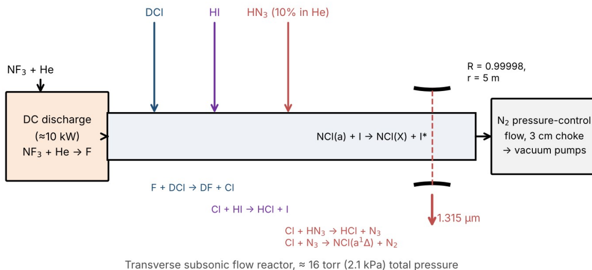
Figure 7. Layout of the first continuous-wave all-gas-phase iodine laser (AGIL), after U.S. Patent 6,459,717. F atoms from an \text{NF}_3/\text{He} discharge are converted to Cl atoms by \text{DCl} . \text{Cl} + \text{HI} supplies ground-state iodine, and \text{Cl} + \text{HN}_3 \rightarrow \text{N}_3 followed by \text{Cl} + \text{N}_3 produces \text{NCl}(a^1\Delta) , which pumps \text{I}(^2\text{P}_{1/2}) in the gain region.
