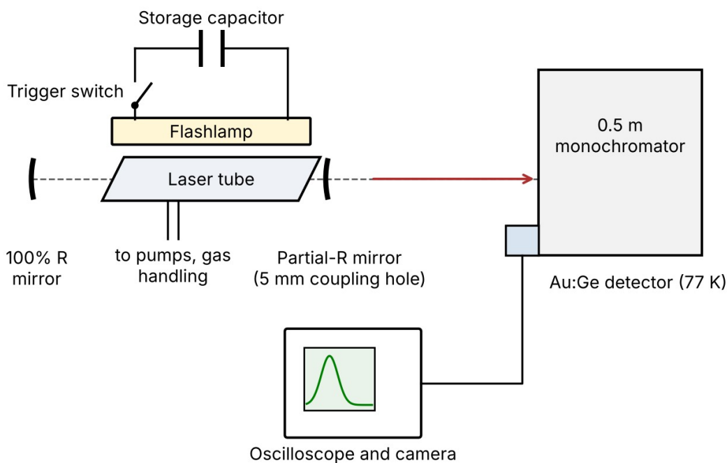
Figure 3. Experimental arrangement of Lin (redrawn from the original hand sketch).
