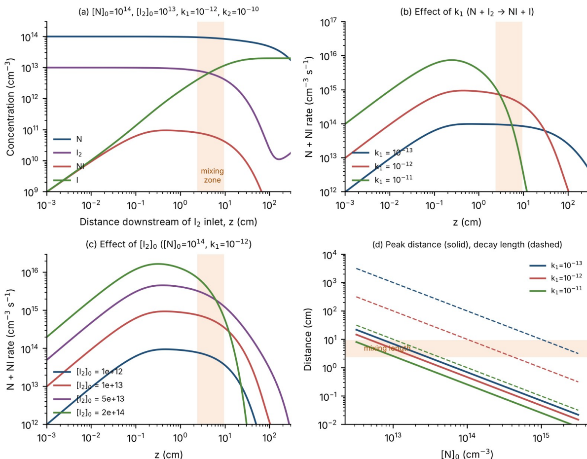
Figure 11. Modeled kinetics of N + I_2 \rightarrow NI + I followed by N + NI in the proposed flow tube (2 torr N_2 , 300 K, plug flow at 10 m/s; k_2 = 10^{-10} \text{ cm}^3 \text{s}^{-1} ; N recombination and wall loss included). (a) Concentrations for [N]_0 = 10^{14} \text{ cm}^{-3} , [I_2]_0 = 10^{13} \text{ cm}^{-3} , k_1 = 10^{-12} \text{ cm}^3 \text{s}^{-1} . (b) N + NI reaction rate for three values of k_1 . (c) Effect of the initial I_2 concentration. (d) Distance to the emission maximum (solid) and decay length v/(k_1[N]) (dashed) as functions of [N]_0 . The shaded band is the estimated I_2 mixing length (2–10 cm).
