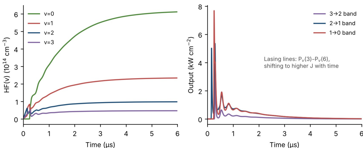
Figure 2. Pulsed F + H_2 \rightarrow HF laser modeled with measured rate data. Left: HF(v) populations. Right: output on the 3→2, 2→1, and 1→0 bands. Conditions: 300 K; 0.13 kPa (1 torr) H_2 with He diluent; 1 \times 10^{15} \text{ cm}^{-3} F atoms formed instantly at t = 0 ; F + H_2 rate constant 2.5 \times 10^{-11} \text{ cm}^3 \text{ s}^{-1} with f_1 : f_2 : f_3 = 0.31 : 1 : 0.47 ; HF-HF V-T 1.7 \times 10^{-12} \text{ cm}^3 \text{ s}^{-1} (ref. 15); HF-HF V-V 1 \times 10^{-11} \text{ cm}^3 \text{ s}^{-1} (order-of-magnitude estimate); 50 cm gain length; 80% output coupler. Lasing is taken on the highest-gain P-branch line of each band, with the rotational populations in equilibrium.
