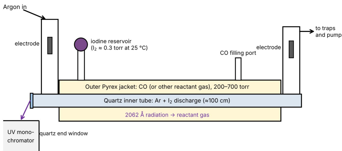
Figure 8. The Harteck–Reeves–Thompson photochemical iodine lamp (redrawn after Fig. 2 of ref. 18). Argon carries iodine vapor from the reservoir through the 100 cm quartz inner tube, where an electrode discharge excites the 2062 Å line. The reactant gas (CO) fills the surrounding Pyrex jacket, and a quartz end window lets a UV monochromator monitor the output.
