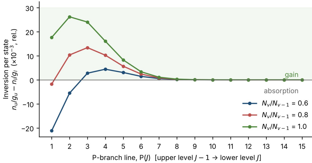
Figure 1. Partial inversion on HF P-branch lines ( B \approx 20.9 \text{ cm}^{-1} , T = 300 \text{ K} ) for three ratios of total vibrational population. Lines above zero have gain even when the vibrational levels are not inverted. (Added in the 2026 revision.)
