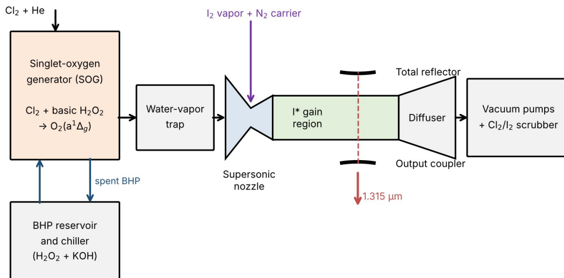
Figure 6. Layout of a supersonic chemical oxygen–iodine laser (COIL). Singlet oxygen made from \text{Cl}_2 and basic hydrogen peroxide passes through a water-vapor trap, is mixed with \text{I}_2 at the nozzle, and pumps atomic iodine in the gain region; the resonator axis is perpendicular to the flow.
