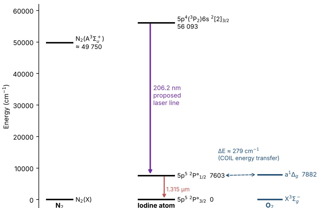
Figure 4. Energy levels relevant to the proposed N + NI iodine laser: the 206.2 nm transition from \text{I}(6s\ ^2[2]_{3/2}) to \text{I}(^2\text{P}_{1/2}) , the 1.315 \mu\text{m} \text{I}(^2\text{P}_{1/2}) \rightarrow \text{I}(^2\text{P}_{3/2}) transition, \text{N}_2(\text{A}^3\Sigma_u^+) , and the near-resonant \text{O}_2(a^1\Delta_g) level. (Added in the 2026 revision.)
