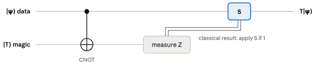
Figure 1. Gate-teleportation circuit for one T gate.
