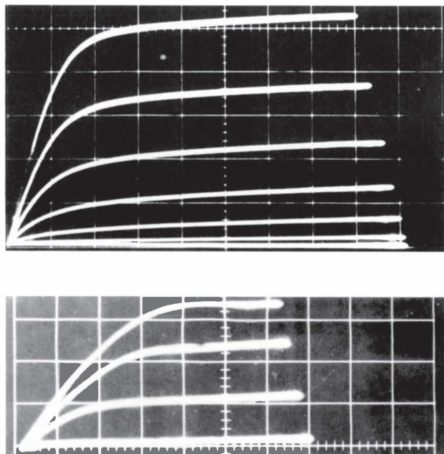
Fig. 3. Current-Voltage characteristics of test FETs. The plots show: (a) recessed gate device; (b) uniform channel device. Vertical is 0.2 \text{ mA/div.} ; and horizontal is 0.5 \text{ V/div.} ; 0.5 \text{ V/step} .
