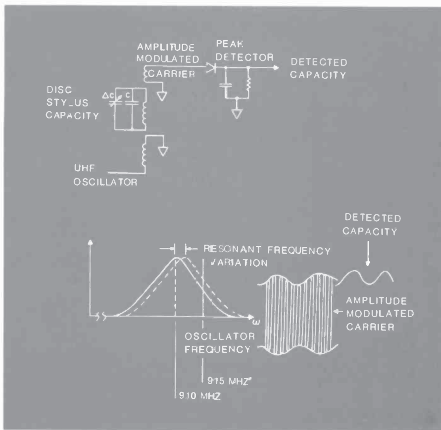
Fig. 5. Disc-stylus capacitance is made part of a circuit resonant at ~910 MHz. As the capacitance changes, the resonant frequency changes, giving rise to a variation in the response of the circuit to a 915-MHz signal and providing amplitude modulation of this signal. The modulation is stripped off by a diode detector to provide a voltage that rises and falls as the disc surface rises and falls under the stylus.
