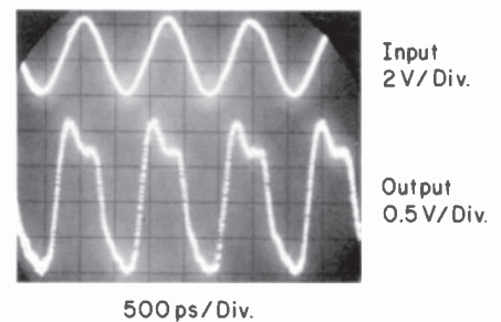
Fig. 7. Response of an inverter to a 950-MHz sinewave input signal. Sharpening of the rise and fall times can be seen in the output pulse.
