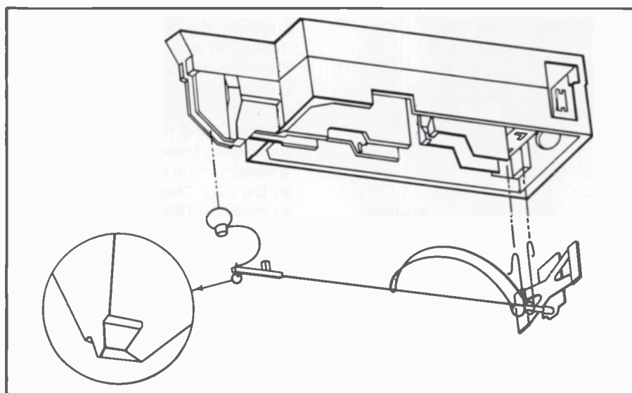
Fig. 5. The stylus cartridge is composed of the diamond stylus, the flylead, the tipholder, the aluminum tube, the arm-stretcher coupler, and a clamp spring. This assembly is user-replaceable.
