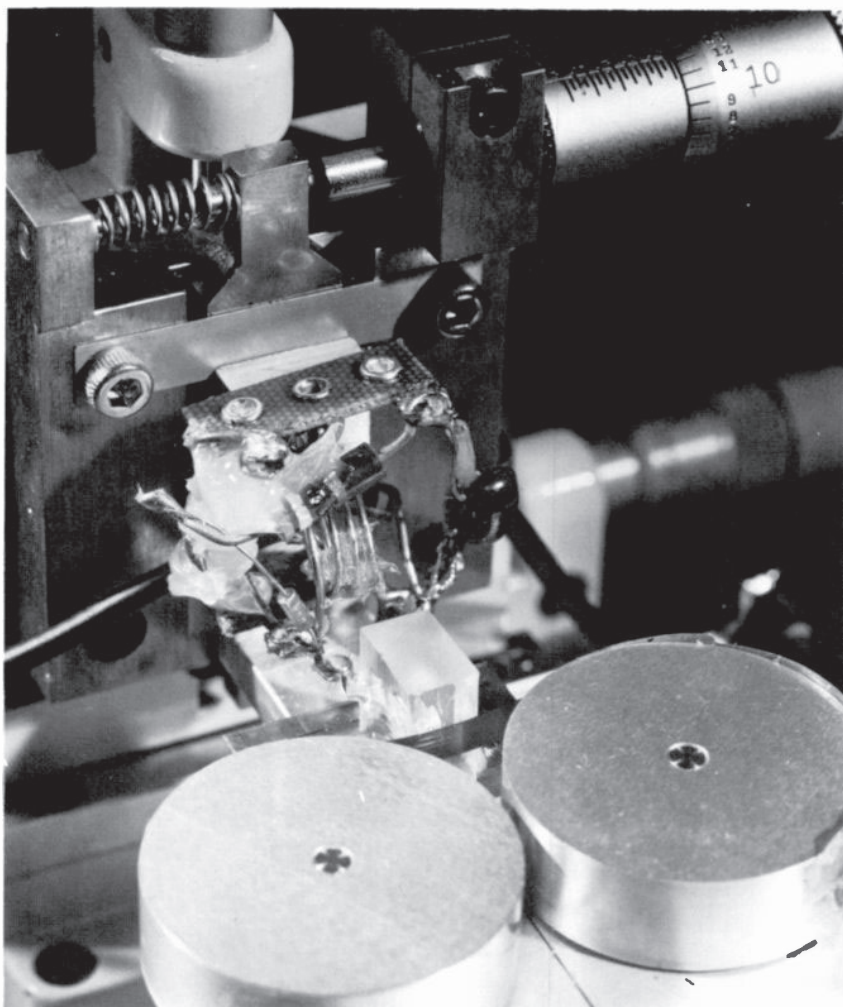
Tiny Tester. Embossed with a microscopic signal pattern, a metallized Mylar tape moves back-and-forth across a stationary "stylus" to test capacitive pickup in this 1967 setup. To make the "stamper" for embossing the Mylar, the electron beam of a scanning electron microscope exposed a line
