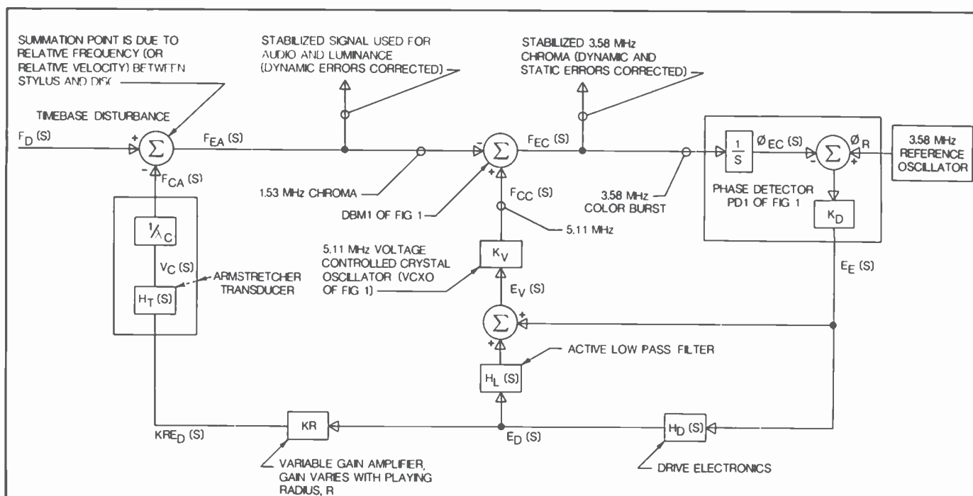
Fig. 4. Time-base-correction system.
