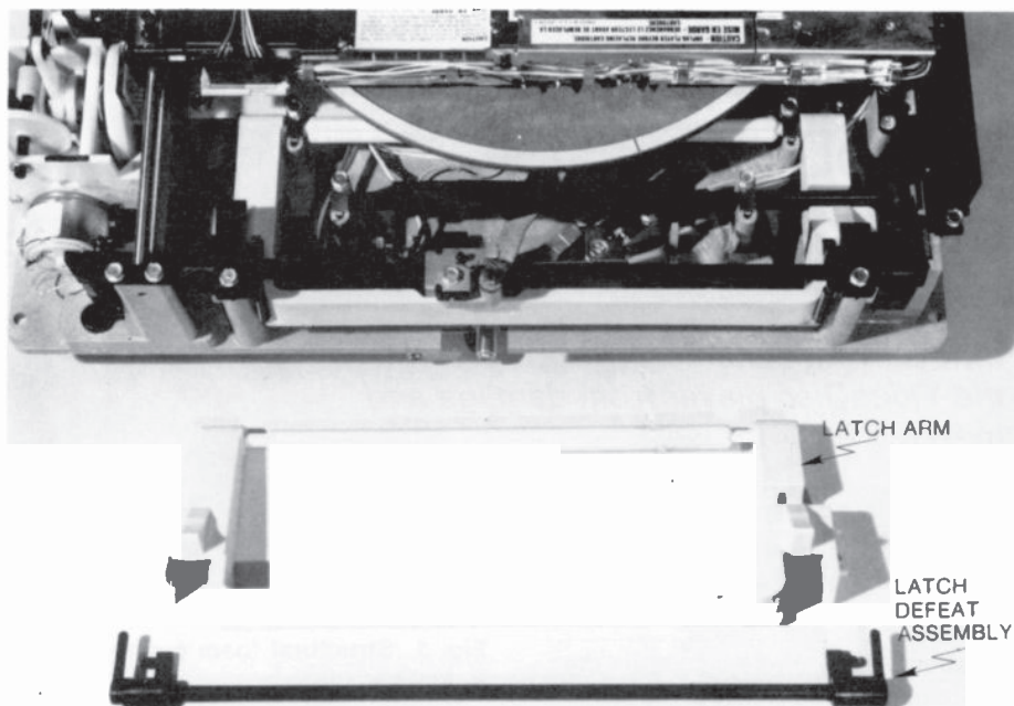
Fig. 2. Caddy loading and unloading functions remove the disc from the caddy for playing and reload disc into caddy after play.
