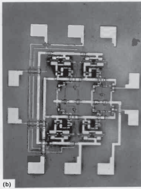
Fig. 5. Photomicrographs of GaAs ICs. (a) Ring oscillator—fan-in = 2, fan-out = 2; (b) D-type master/slave flip-flop; and (c) 2-bit A/D converter. The 1.0\text{-}\mu\text{m} gate-length devices are used in A/D and the 1.5\text{-}\mu\text{m} gate-length devices are used in ring oscillators and flip-flops.
