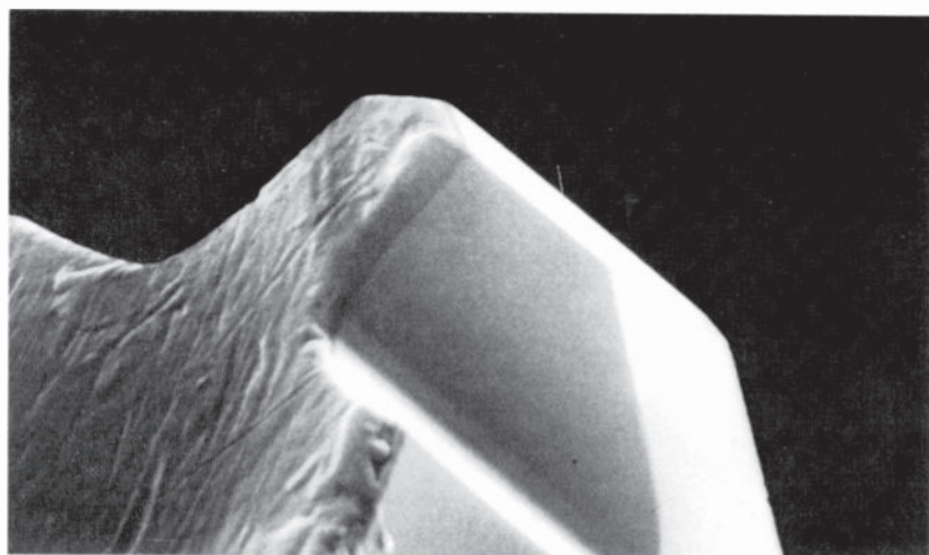
Fig. 2. Stylus tip. This is a scanning electron microscope photograph of the stylus tip magnified 9000 times. The tip of the stylus that plays the disc is too small to be seen with an optical microscope and must be observed using the higher magnification of a sophisticated scanning electron microscope. The metal electrode coated on the diamond surface is used as one side of the capacitance pickup of the VideoDisc signal with the conductive disc used as the second side. Sophisticated
