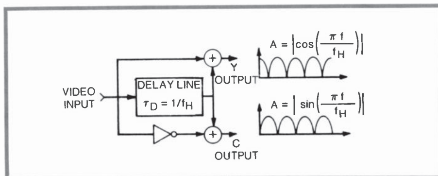
Fig. 1. Basic comb-filter circuit. The resulting amplitude responses for luminance (Y) and chrominance (C) outputs are shown on the right.
