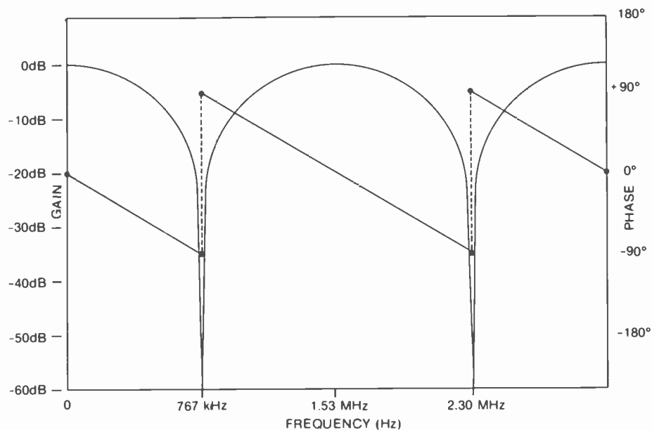
Fig. 3. The amplitude and phase response of the 1-H output, gives the necessary 180-degree phase inversion at the chrominance subcarrier. This phase relationship is required to substitute "previous" line video for defects occurring on the "present" line.
