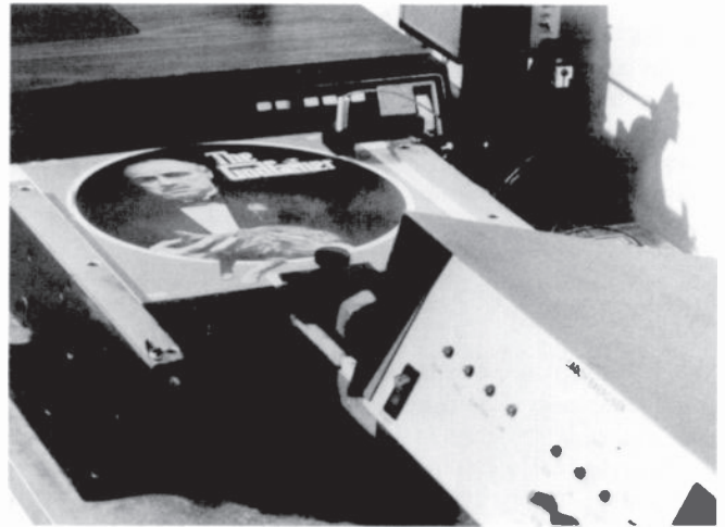
Fig. 1. Caddy exerciser for player life-test cycling.
