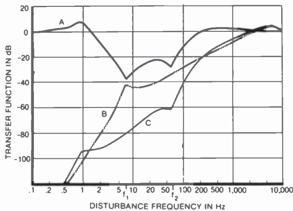
Fig. 5. Time-base-correction system transfer functions.
