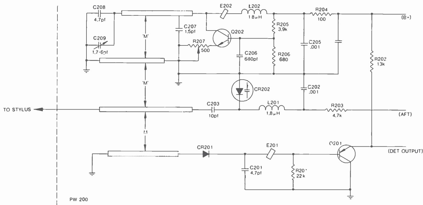
Fig. 6. Resonator schematic. Energy from a fixed 915-MHz oscillator is coupled, via the resonant circuit, to detector loop. The sensitivity of the resonance change in capacitance transforms a change in energy to the detector at the signal rate.
