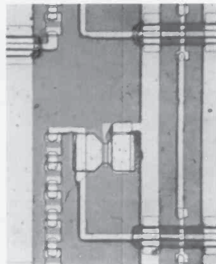
Fig. 4. Photomicrograph of a two-level interconnect pattern. Polyimide dielectric layer used for isolating the crossovers. The width of the smallest line is 3.0\text{ }\mu\text{m} . Polyimide islands as small as 7.5 to 10\text{ }\mu\text{m} were used.
