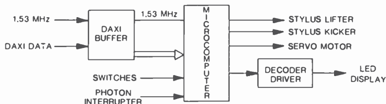
Fig. 1. Digital control system. The principal parts of the control system are shown above. The system comprises three custom integrated circuits with the microcomputer as the main control element. The stylus-lifter signal is used to lift or lower the stylus. The stylus-kicker signal energizes a kicker coil that kicks the stylus forward or backward several microns. The servo-motor signal actuates a motor that moves the stylus carriage backward and forward. The switch inputs include the rapid access, visual search, pause, and load functions. The photon interrupter consists of a light beam that is interrupted by the arm every time the arm moves a distance equal to one minute. The resultant signal is sent to the microcomputer.
