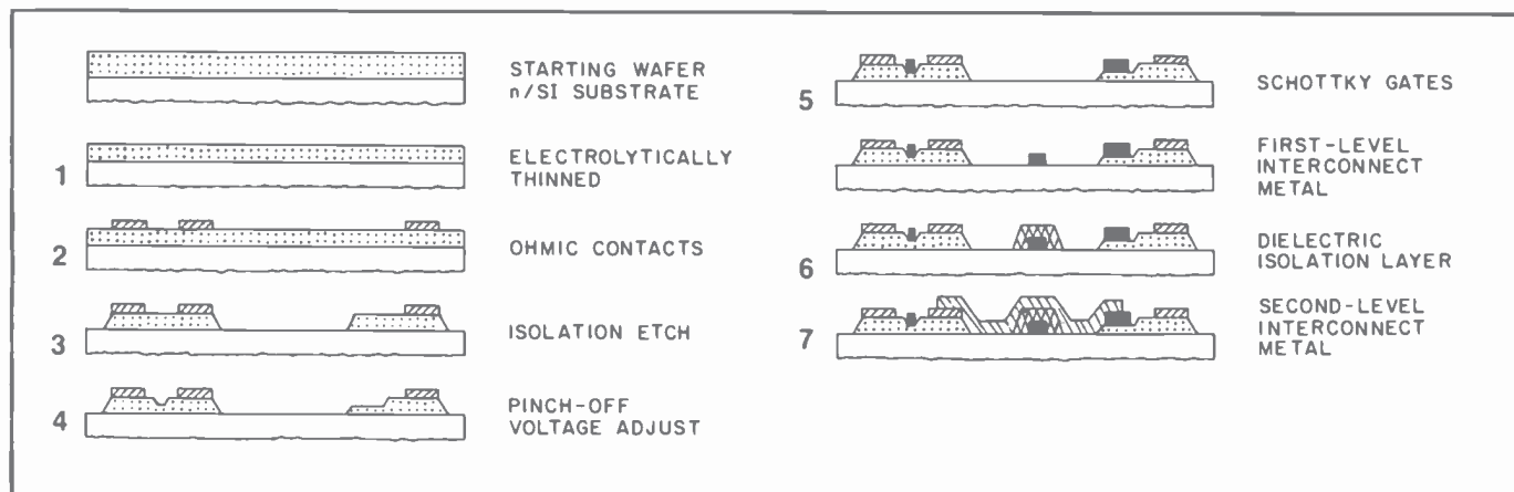
Fig. 2. Process schedule for IC fabrication. It takes seven masking steps to complete the IC.
