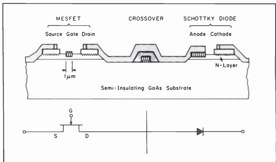
Fig. 1. GaAs IC cross section. A MESFET and a Schottky diode are the active devices. Interconnections with two-level metal lines and dielectric isolation layer for crossovers are also shown.
