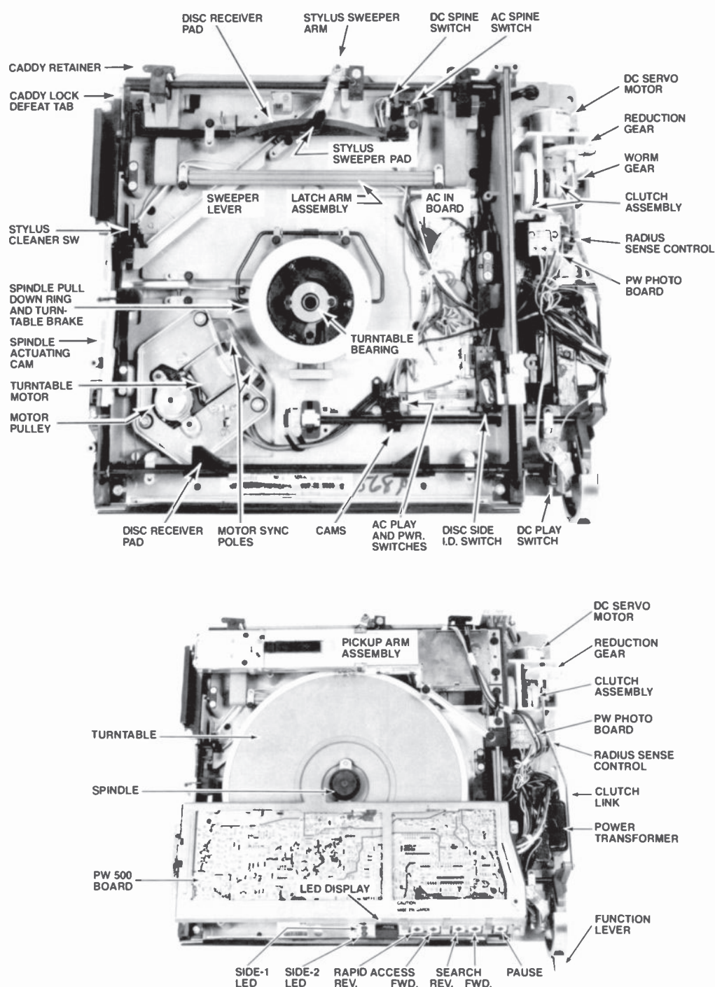
Fig. 7. Top view of the VideoDisc player with the cabinet shell removed. The upper view also shows the control board (PW500), turntable, and pickup-arm assembly removed (for clarity).
