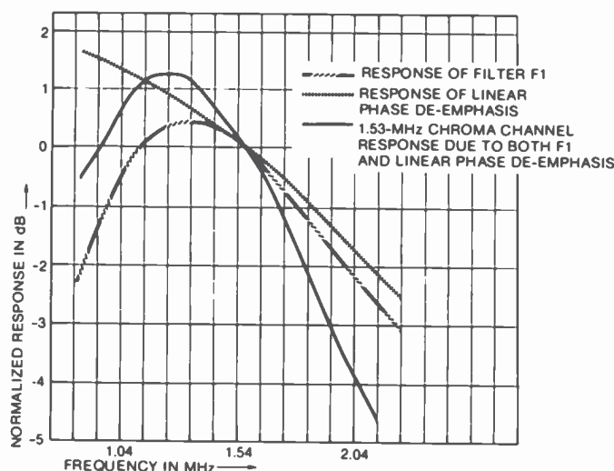
Fig. 2. Chroma responses.
