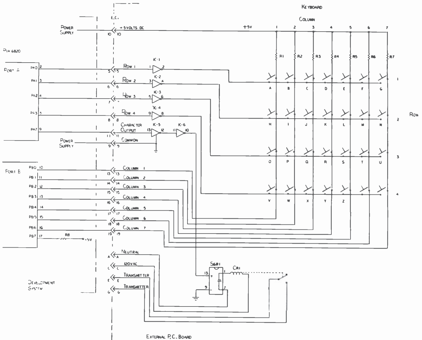
Fig. 3. This schematic diagram shows the hardware interconnections between the PIA 6820 and the 4 x 7 keyboard. One 7404 hex buffer, a solid state relay, a control relay, and 28 single-pull-single-throw push buttons were used.
