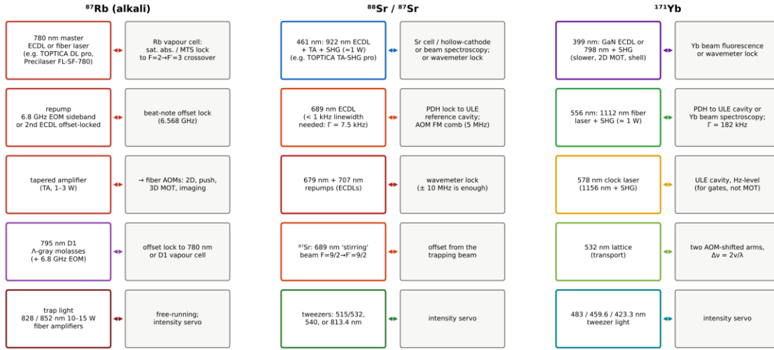
Figure 3. Laser sources (left of each pair) and frequency references or distribution (right) for Rb, Sr and Yb machines.
