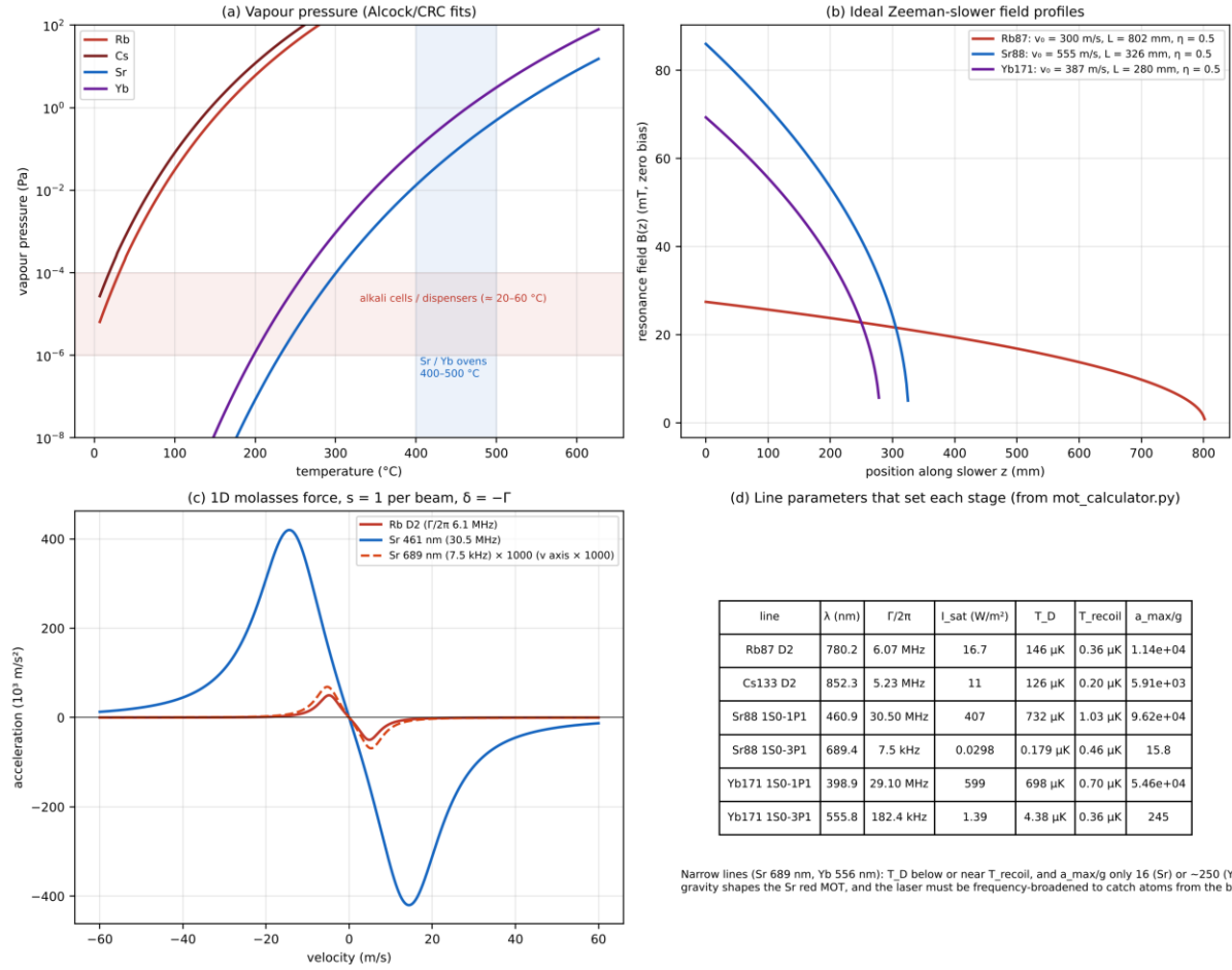
Figure 4. (a) Vapor pressure of Rb, Cs, Sr and Yb. (b) Ideal Zeeman-slower profiles. (c) 1D molasses acceleration versus velocity for broad and narrow lines. (d) Line parameters for each stage. All values computed by mot_calculator.py.
