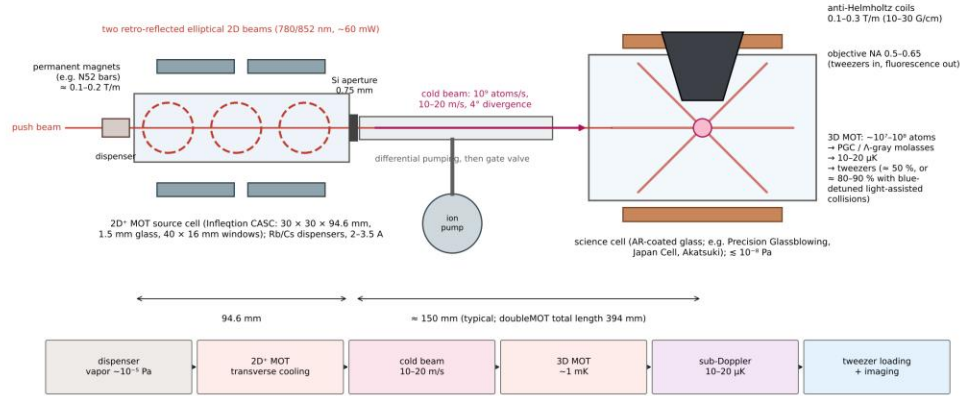
(a) Compact alkali source: 2\text{D}^+ MOT cell \rightarrow 3D MOT in the science cell \rightarrow tweezers loaded directly (Rb or Cs)
