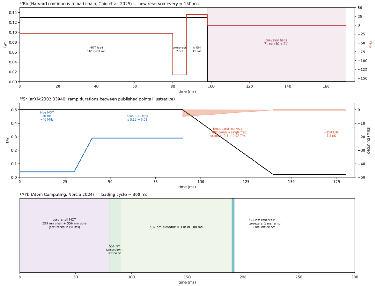
Figure 5. Loading sequences. Rb: Harvard continuous-reload chain (published durations and detunings). Sr: ^{88}\text{Sr} example (published end points; ramp shapes between them illustrative). Yb: Atom Computing core-shell MOT and elevator (published durations).
