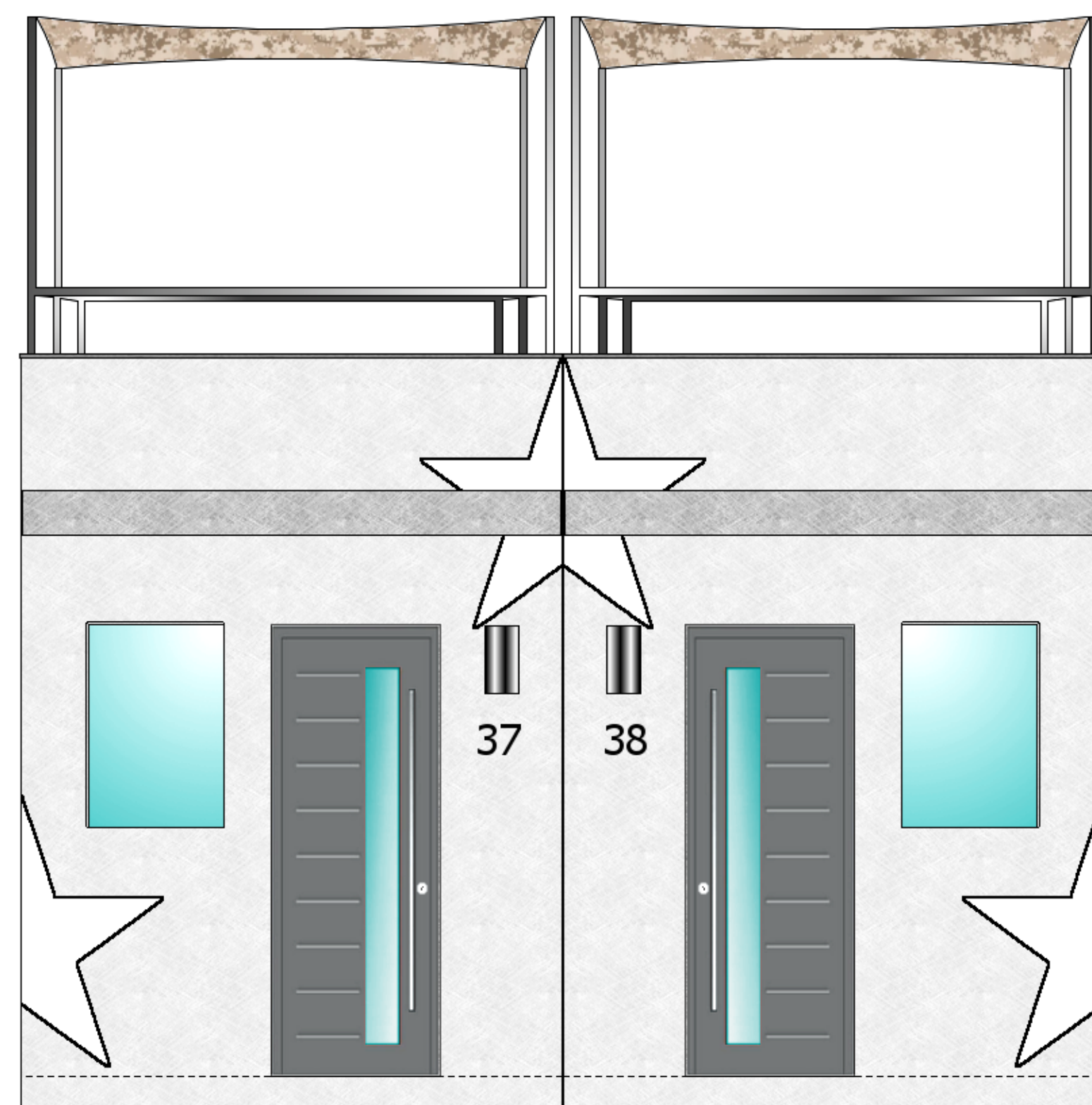
FRONT ELEVATION VIEW of SIDE by SIDE UNITS
