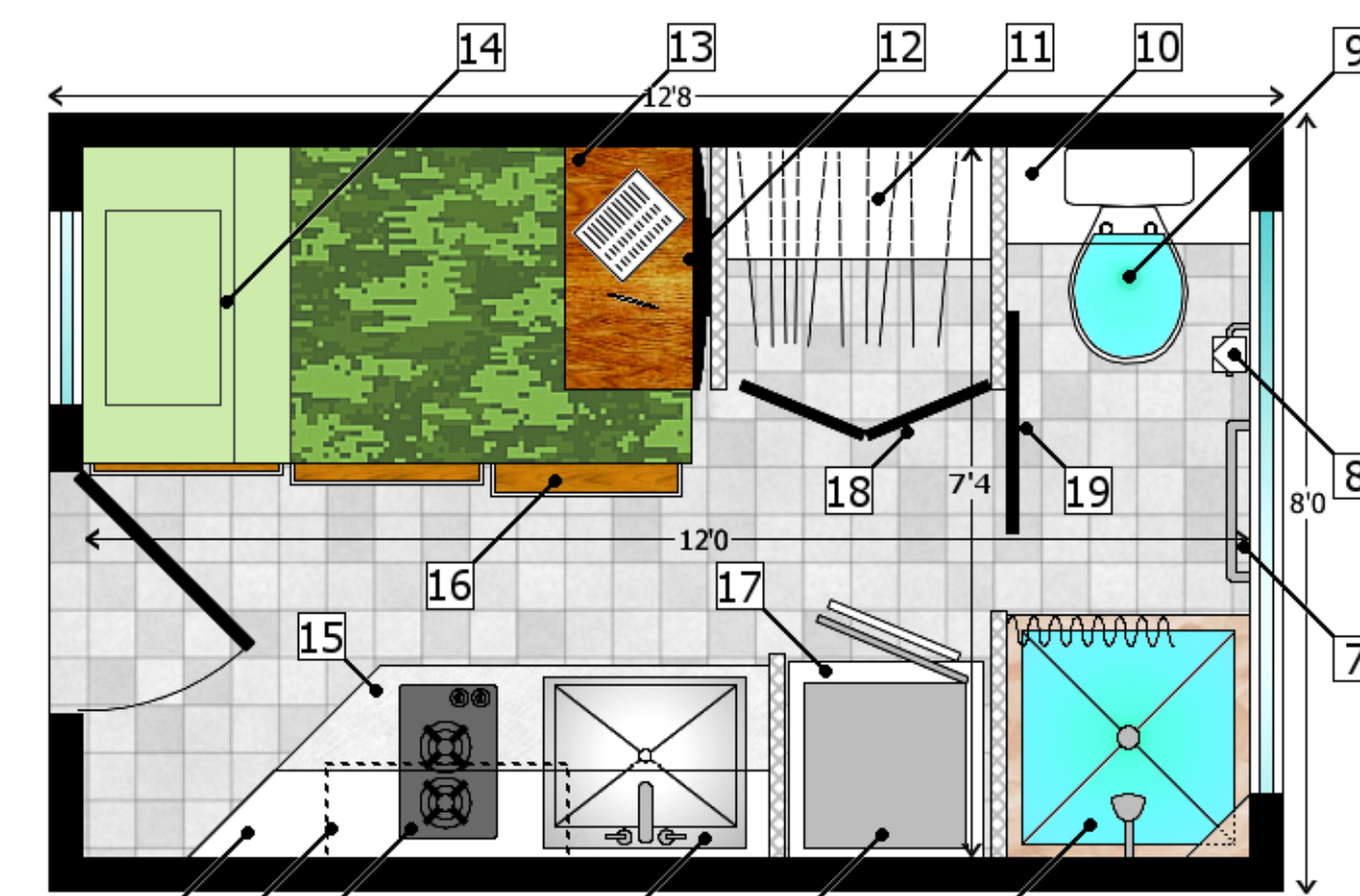
BP2-01 CASTLETTE FLOOR PLAN 88 SqFt.
