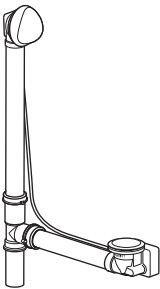
Fig. C Traditional TurnControl Tubular Rough-In Complete Unit
