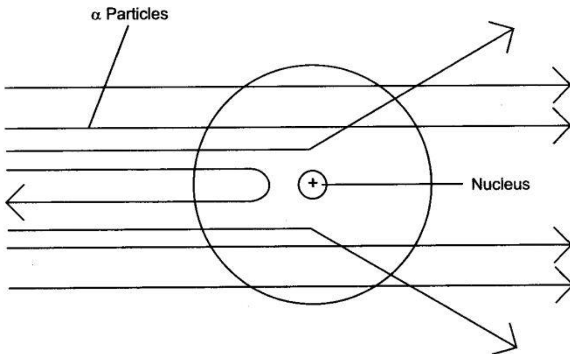
Rutherford's Model
