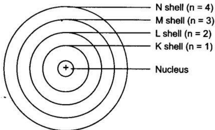
Bohr's Model
