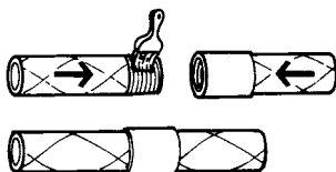
Figure 2 T.A.B. (Threaded and Bonded) Joint
