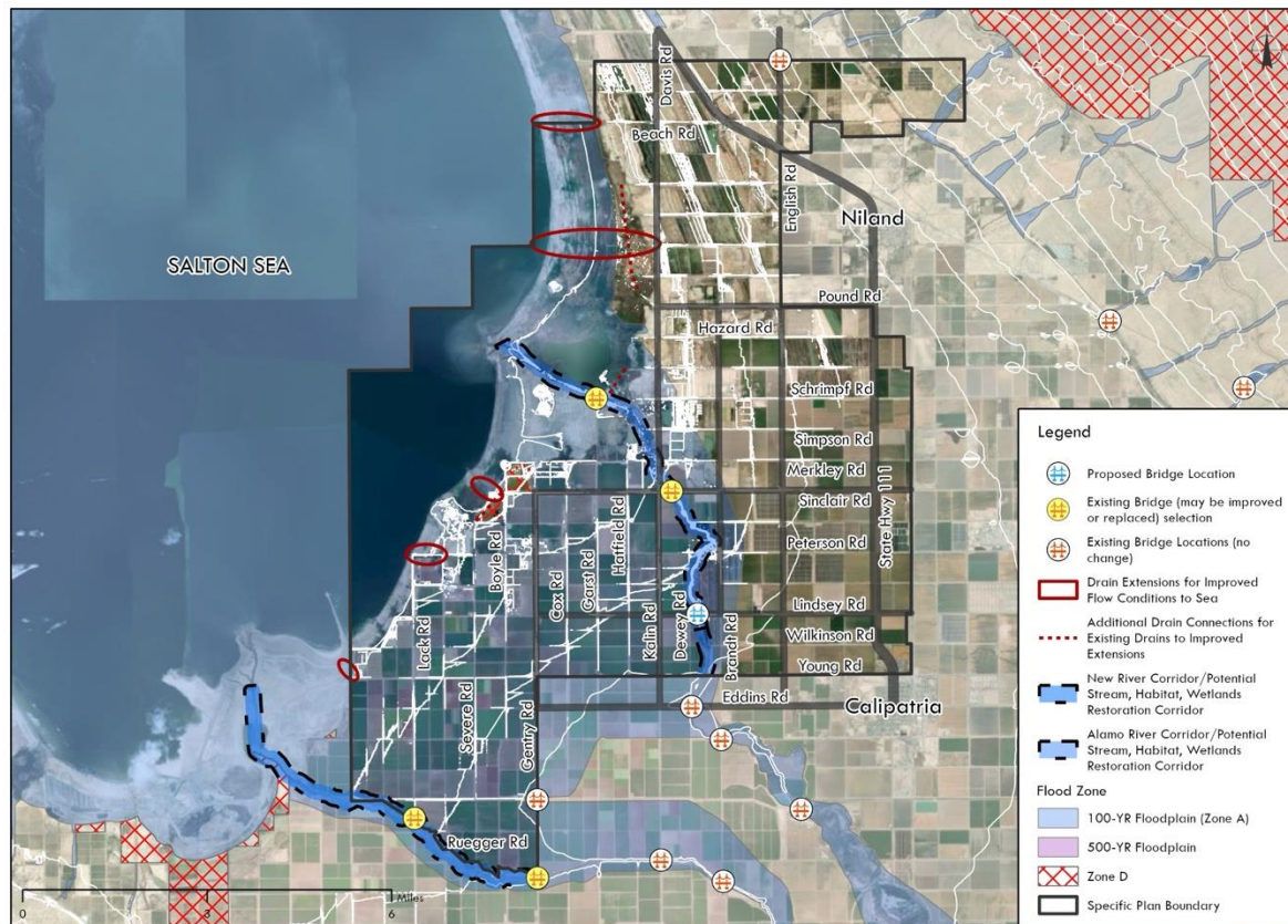
Figure 6-4, Drainage Infrastructure Opportunities
