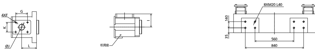
HOPPER MOUNTING DIMENSION
