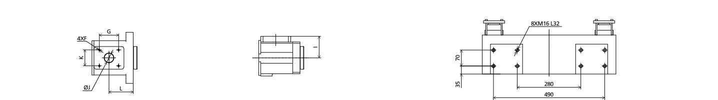
HOPPER MOUNTING DIMENSION
