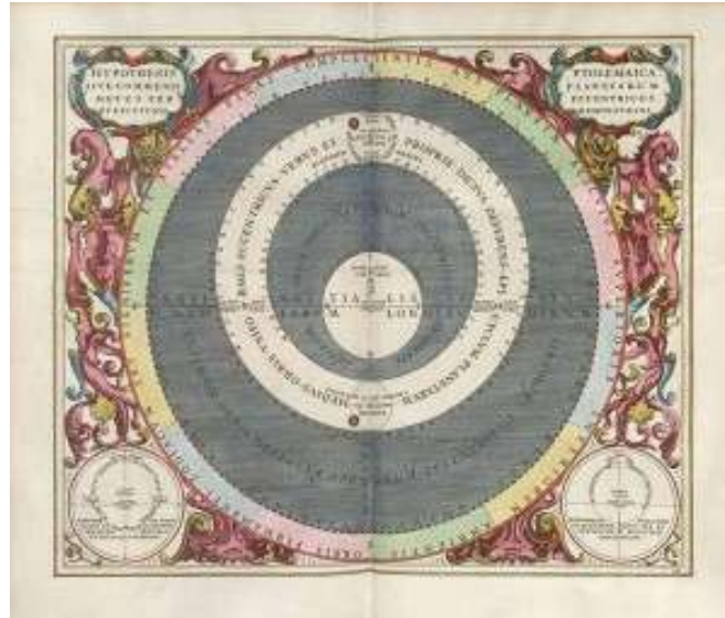
Andreas Cellarius hypothesis, showing the planetary motions.
