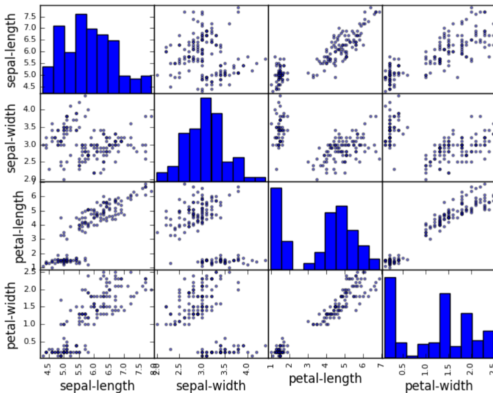
Scatterplot Matrix
