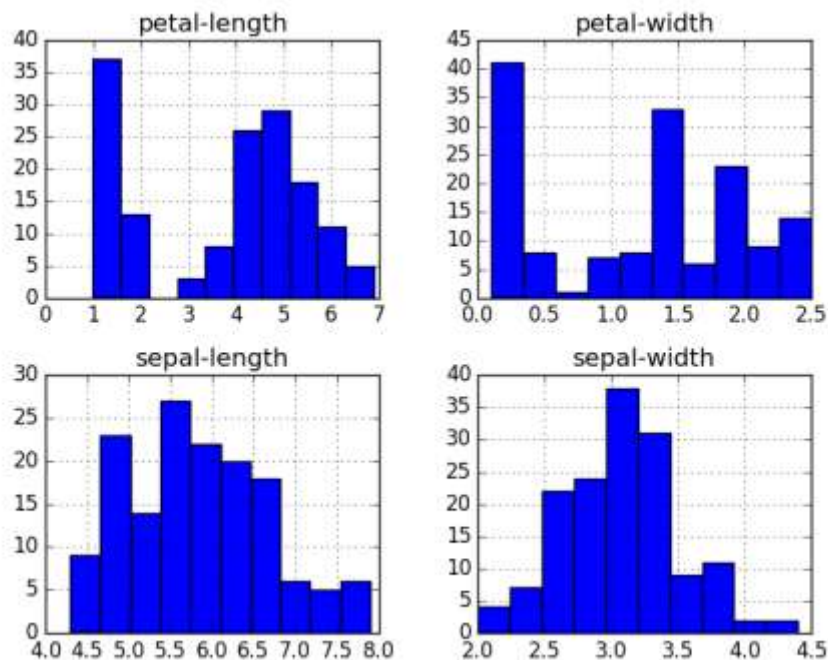
Histogram Plots
