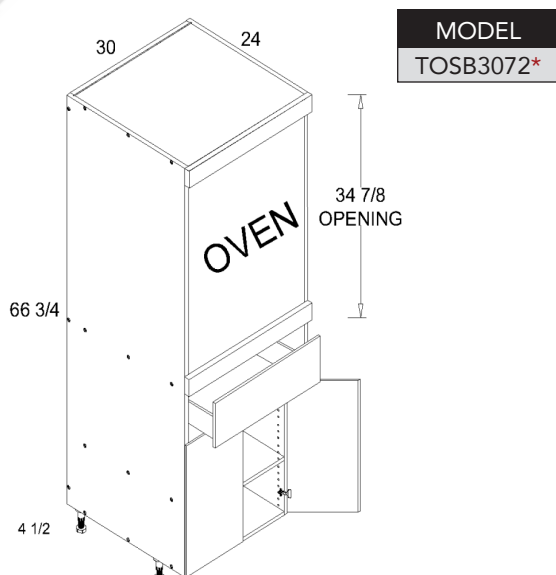
Tall Single Oven Two Door One Drawer Utility
