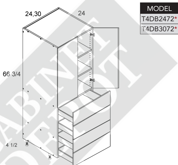
Tall Two Door Four Drawer Utility
