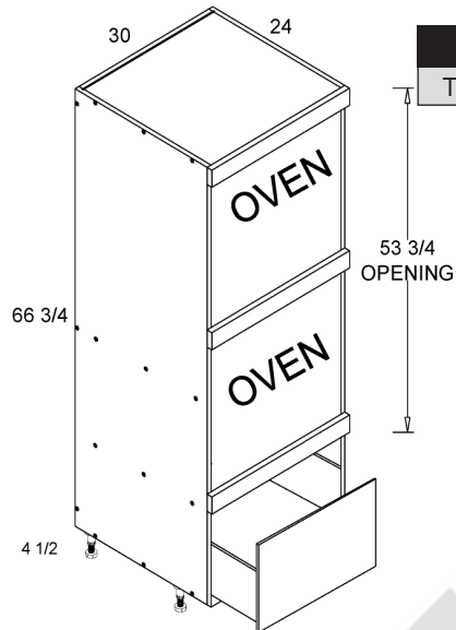
Tall Double Oven One Drawer Utility
