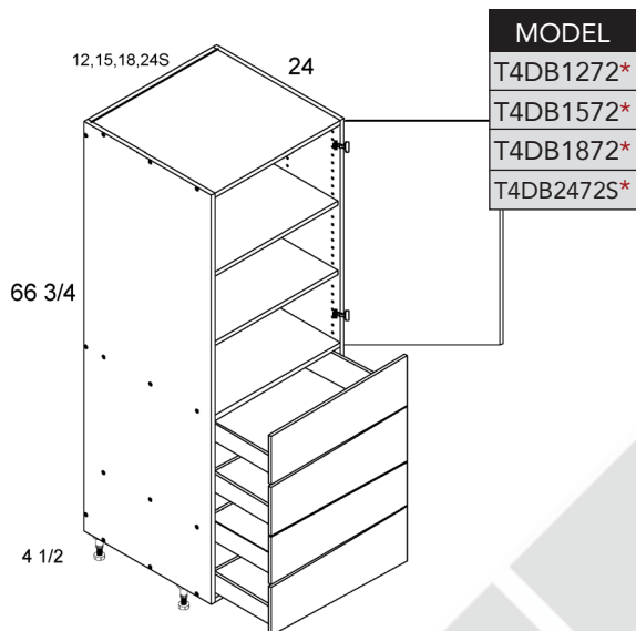
Tall One Door Four Drawer Utility
