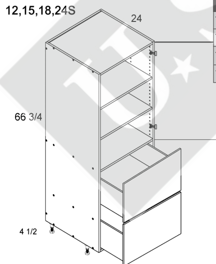
Tall One Door Two Drawer Utility
